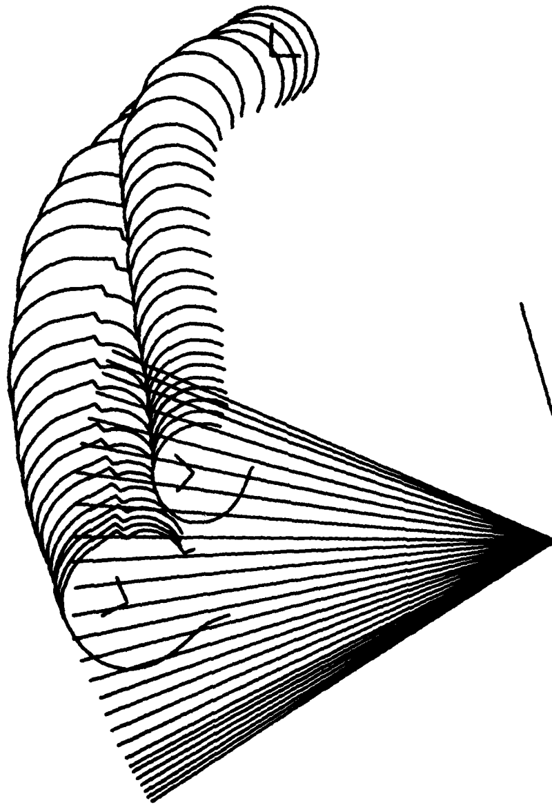
FIGURE A-22. Tracing of head movement of adult dummy holding infant dummy in lap.
