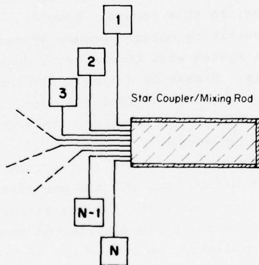
Figure 4-10. Star system configuration.
