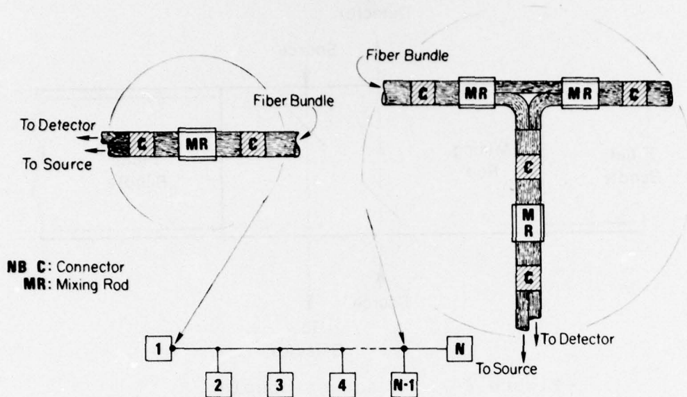
Figure 4-8. Tee system configuration.
