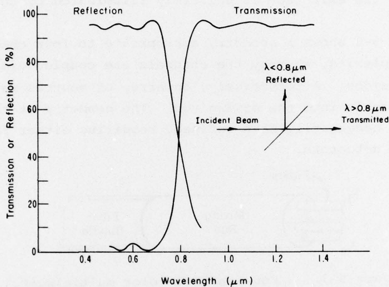
Figure 5-2. Filter characteristics for use with WDM.
