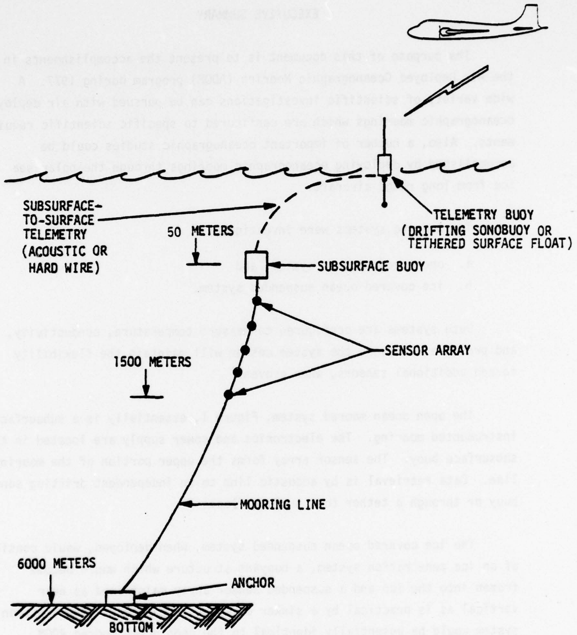
Figure 1. Open Ocean Moored System
