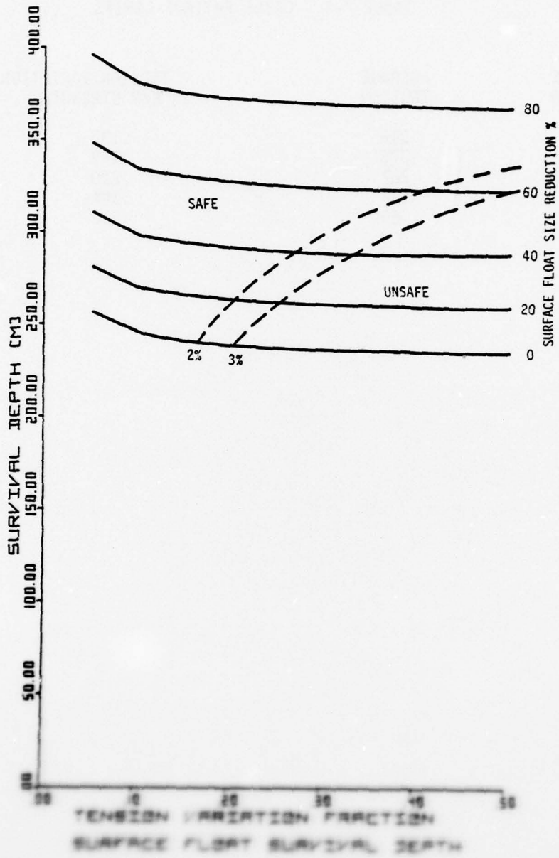
Figure 2-4. Surface Float Depth
