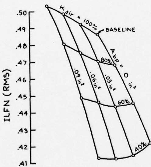
FIGURE 4 YC-14 MAIN GEAR PARAMETER VARIATION LANDING CONFIGURATION
