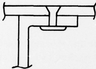
FIGURE 27 WING UPPER SURFACE SKIN - STRINGER ATTACHMENT
