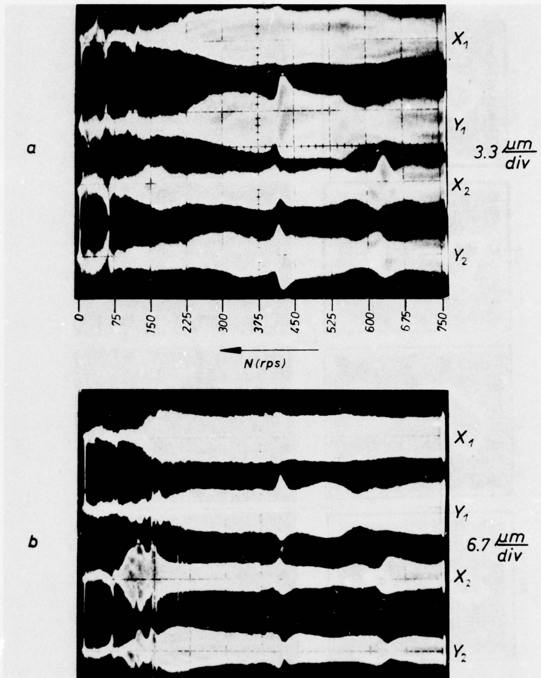
FIGURE 85. AMPLITUDE SCANS DURING COASTDOWN.-JOURNAL FOIL BEARING LLF-2J (OCTAGONALLY BENT BACKING AND 2-1/4 INNER TURNS. ONE STEEL FOIL PER BEARING, L \times D \times t_f = 20 \times 30 \times 0.054 mm. JOURNAL DIAMETER = 29.872 mm, FOIL-CARTRIDGE BORE = 30.61 mm).- (a) WITHOUT ADDED UNBALANCE: (b) WITH ASYMMETRIC UNBALANCE U_1 = 19.3 \mu\text{m} . N AND U_2 = 23.2 \mu\text{m} . N
