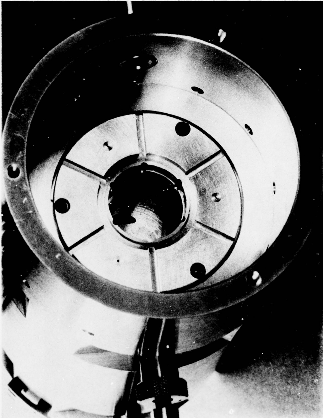
FIGURE 4. VIEW OF HOUSING AND AIR BEARING
