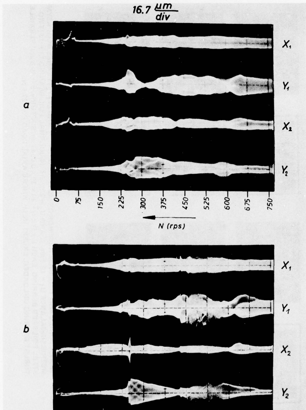
FIGURE 76. AMPLITUDE SCAN DURING COASTDOWN WITH ASYMMETRIC UNBALANCE U_1 = 19.3 \mu\text{m} . N AND U_2 = 23.2 \mu\text{m} . N.-JOURNAL FOIL-BEARING LLF-1J (STEEL FOILS, EACH L \times D \times t_f = 20 \times 30 \times 0.054 \text{ mm} . SIX TURNS, \bar{c} \approx 39.8 \mu\text{m} ).-FLEXIBLE THRUST BEARING UNLOADED. (a) TWO FOILS PER BEARING; (b) ONE FOIL PER BEARING
