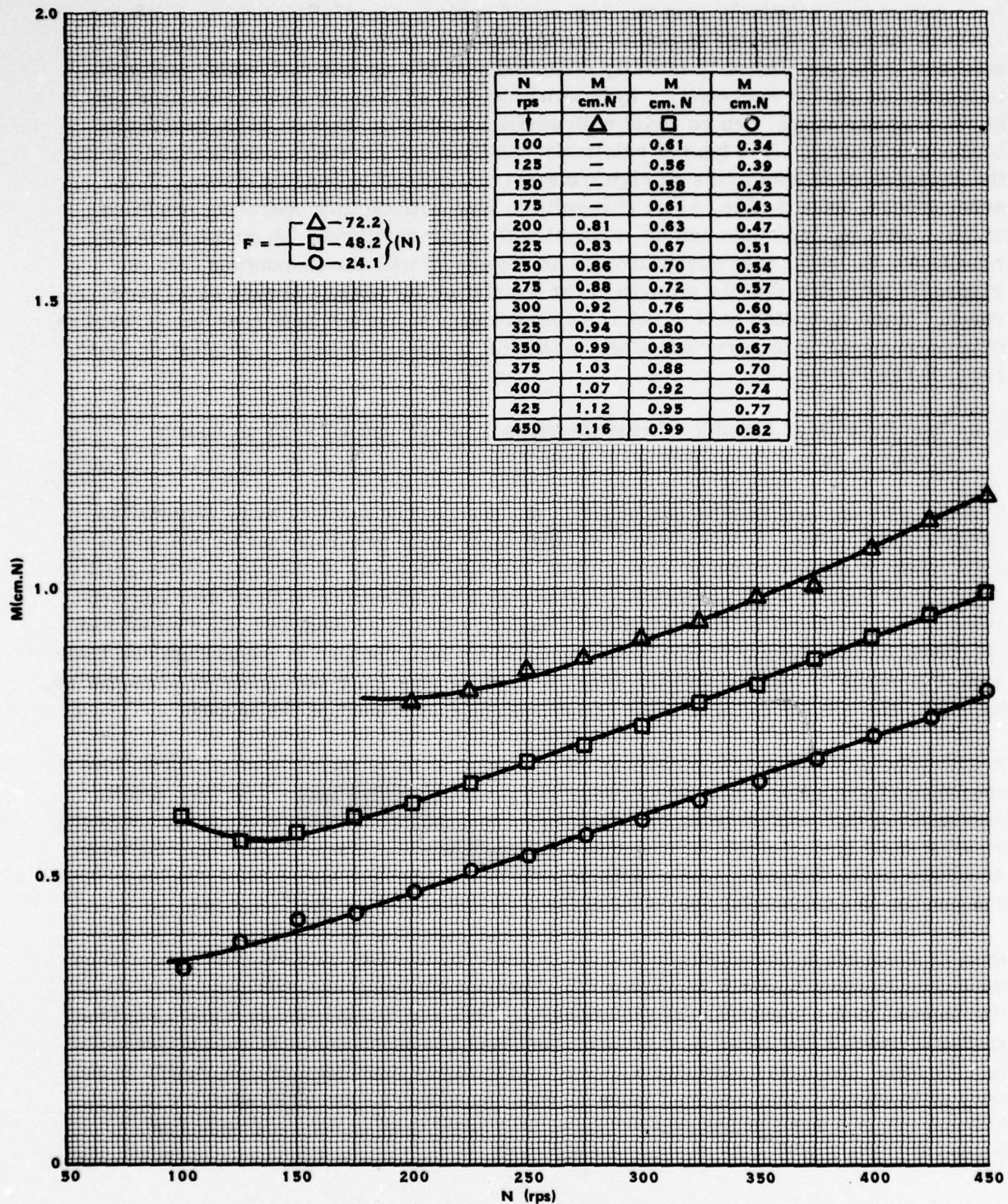
FIGURE 59. FRICTION MOMENT VERSUS SPEED AT CONSTANT LOAD.- FLEXIBLE THRUST BEARING LLF-2T (INCONEL X-750 MEM- BRANE, t_m = 215 \mu\text{m} . Cu-Be SPIDER SPRING, t_p = 200 \mu\text{m} ; \bar{t}_s = 40 \mu\text{m} )
