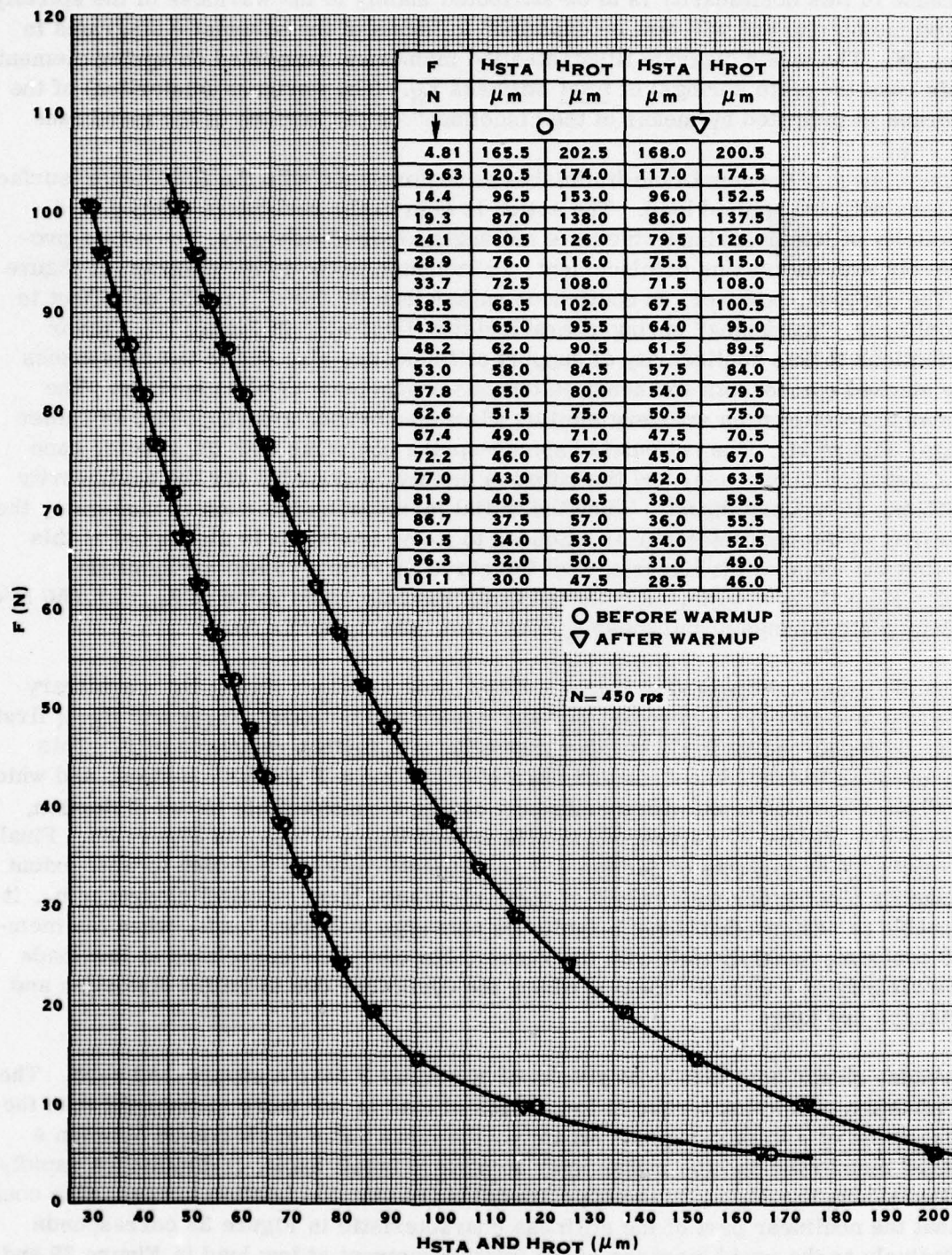
FIGURE 39. DISPLACEMENT OF RUNNER RELATIVE TO SUPPORT PLATE WITH AND WITHOUT ROTATION (DETERMINATION OF CLEARANCE \tilde{h} = H_{ROT} - H_{STA} , FIGURE 37). - FLEXIBLE THRUST BEARING LLF-1T
