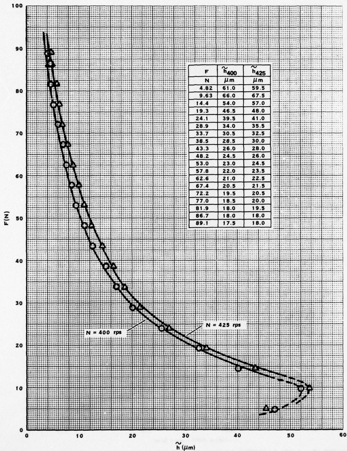
FIGURE 46. LOAD VERSUS CLEARANCE AT N = 400\text{rps} AND N = 425\text{rps} .-FLEXIBLE THRUST BEARING LLF-2T (Cu-Be MEMBRANE, t_m = 230 \mu\text{m} , Cu-Be SPIDER SPRING, t_p = 200 \mu\text{m} ; \tilde{t}_s = 72 \mu\text{m} )
