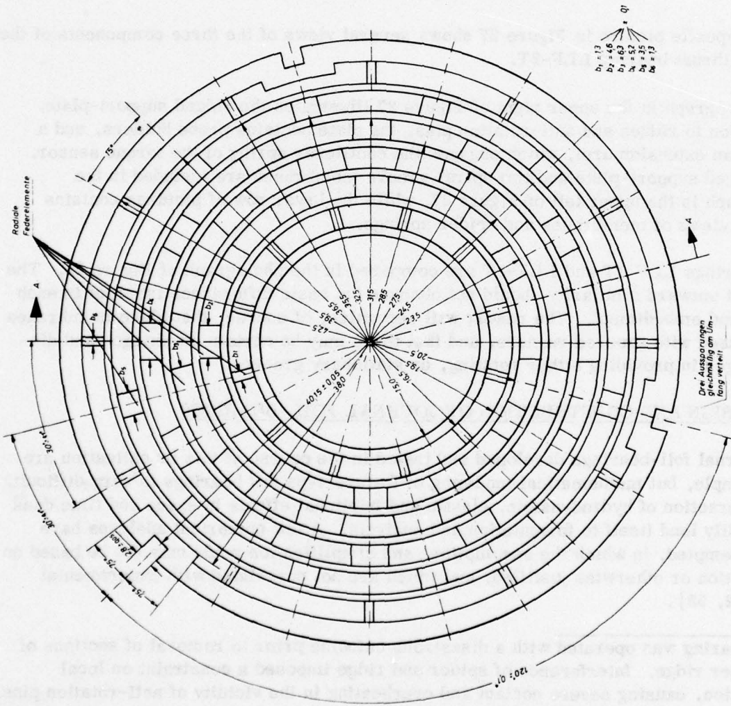
FIGURE 24. SPIDER SPRING OF FLEXIBLE THRUST BEARING LLF-2T
