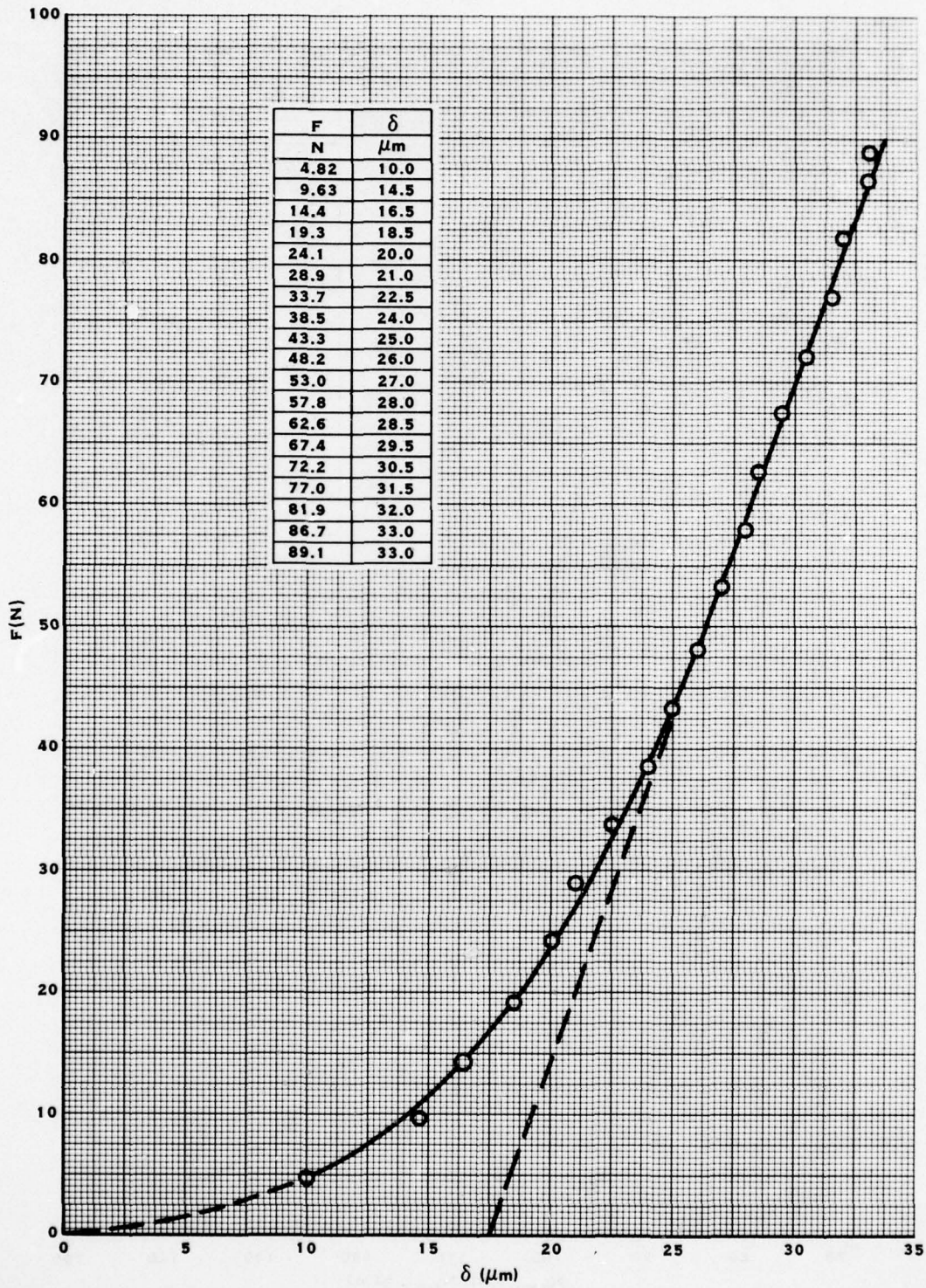
FIGURE 44. STATIC DEFLECTION OF FLEXIBLE THRUST BEARING LLF-2T (INCONEL X-750 MEMBRANE, t_m = 215 \mu\text{m} , Cu-Be SPIDER SPRING, t_p = 200 \mu\text{m} ; \bar{r}_s = 72 \mu\text{m} )
