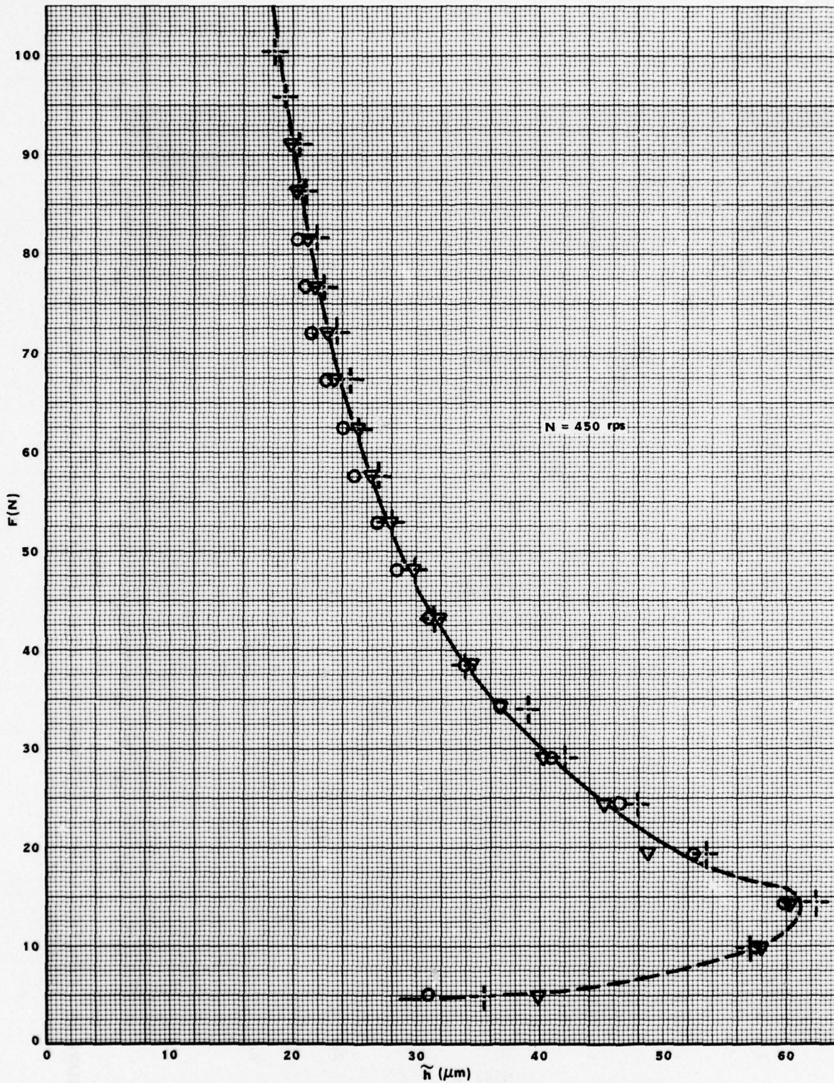
FIGURE 35. LOAD VERSUS CLEARANCE AT N = 450\text{rps} .-FLEXIBLE THRUST BEARING LLF-1T. POINTS DENOTED BY CIRCLES, TRIANGLES AND CROSSES REFER TO RUNS REPEATED UNDER NEARLY IDENTICAL CONDITIONS AND WITH PROGRESSIVE INCREASE OF LOAD (SEE DATA AND REMARKS OF TABLE 1, SECTION 5.1)
