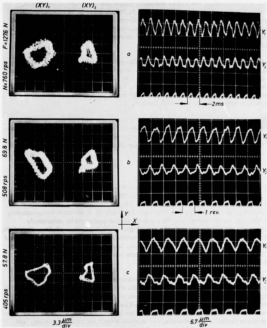
FIGURE 86. TRAJECTORIES AND TIME-BASE RECORDS OF MOTION IN (XY)_{1,2} AND (Y_1Y_2) PLANES WITH ASYMMETRIC UNBALANCE U_1 = 19.3 \mu\text{m} . N AND U_2 = 23.2 \mu\text{m} . N.-JOURNAL FOIL BEARING LLF-2J (OCTAGONALLY BENT BACKING AND 2-1/4 INNER TURNS, ONE STEEL FOIL PER BEARING. L \times D \times t_f = 20 \times 30 \times 0.054 \text{ mm} . JOURNAL DIAMETER = 29.87 mm, FOIL-CARTRIDGE BORE = 30.61 mm).-THRUST LOADS AND SPEEDS AS INDICATED)
