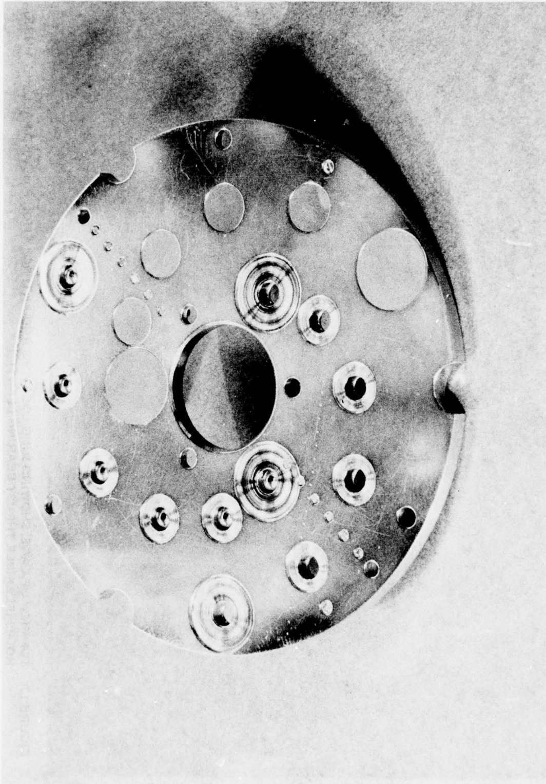
FIGURE 18. VIEW OF UNDERSIDE OF CAGE, SHOWING ARRANGEMENT FOR RETENTION OF BALLS AND SPRING PLATES (FLEXIBLE THRUSTR BEARING LLF-1T)
