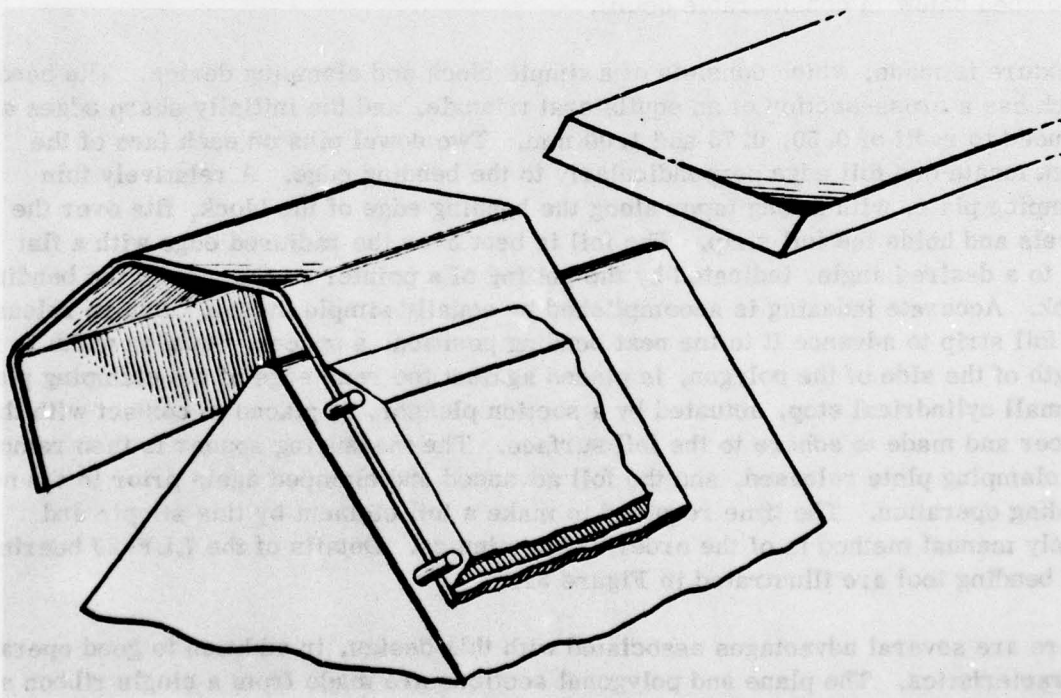
FIGURE 31. JOURNAL FOIL-BEARING LLF-2J.-FOIL ELEMENT WITH QUASI-OCTAGONAL SECTION AND SCHEMATIC DIAGRAM OF BENDING TOOL
