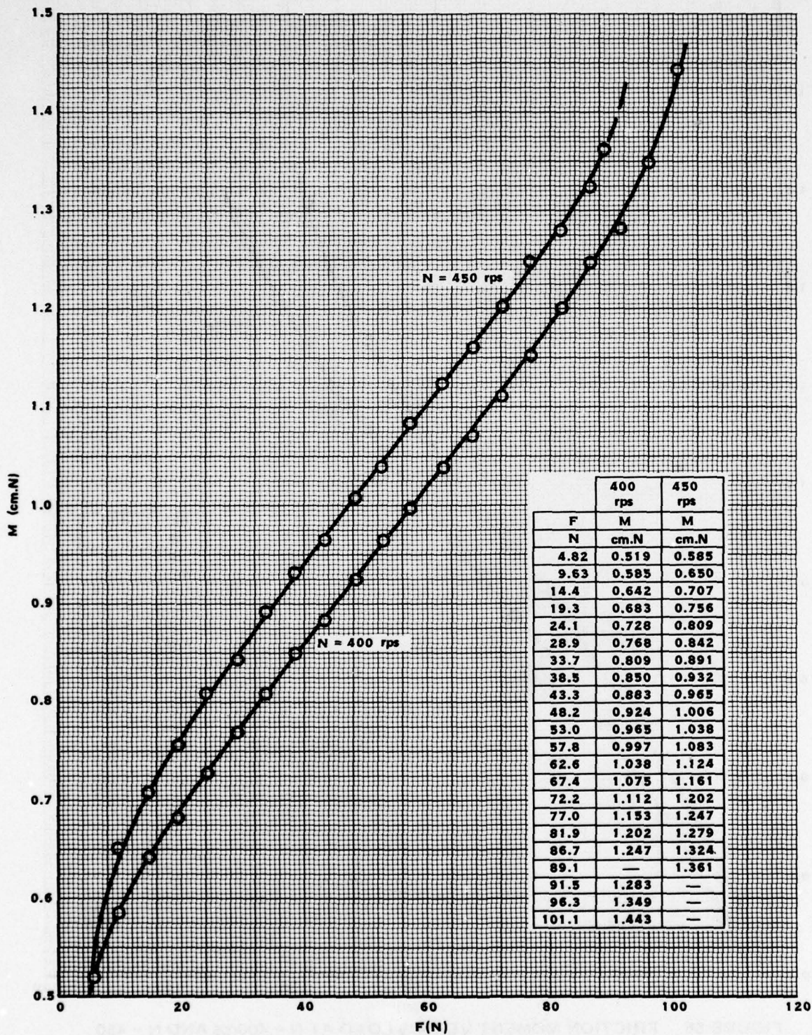
FIGURE 55. FRICTION MOMENT VERSUS LOAD AT N = 400rps AND N = 450rps.- FLEXIBLE THRUST BEARING LLF-2T (INCONEL X-750 MEMBRANE, t_m = 215 \mu\text{m} . Cu-Be SPIDER SPRING, t_p = 200 \mu\text{m} ; \bar{t}_s = 40 \mu\text{m} )
