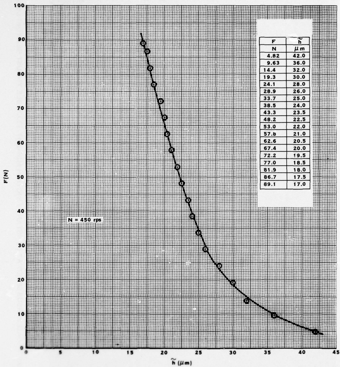
FIGURE 42 LOAD VERSUS CLEARANCE AT N = 450\text{ rps} . FLEXIBLE THRUST BEARING LLF-2T (INCONEL X-750 MEMBRANE, t_m = 215 \mu\text{m} , Cu-Be SPIDER SPRING, t_s = 200 \mu\text{m} , \bar{T}_s = 72 \mu\text{m} )
