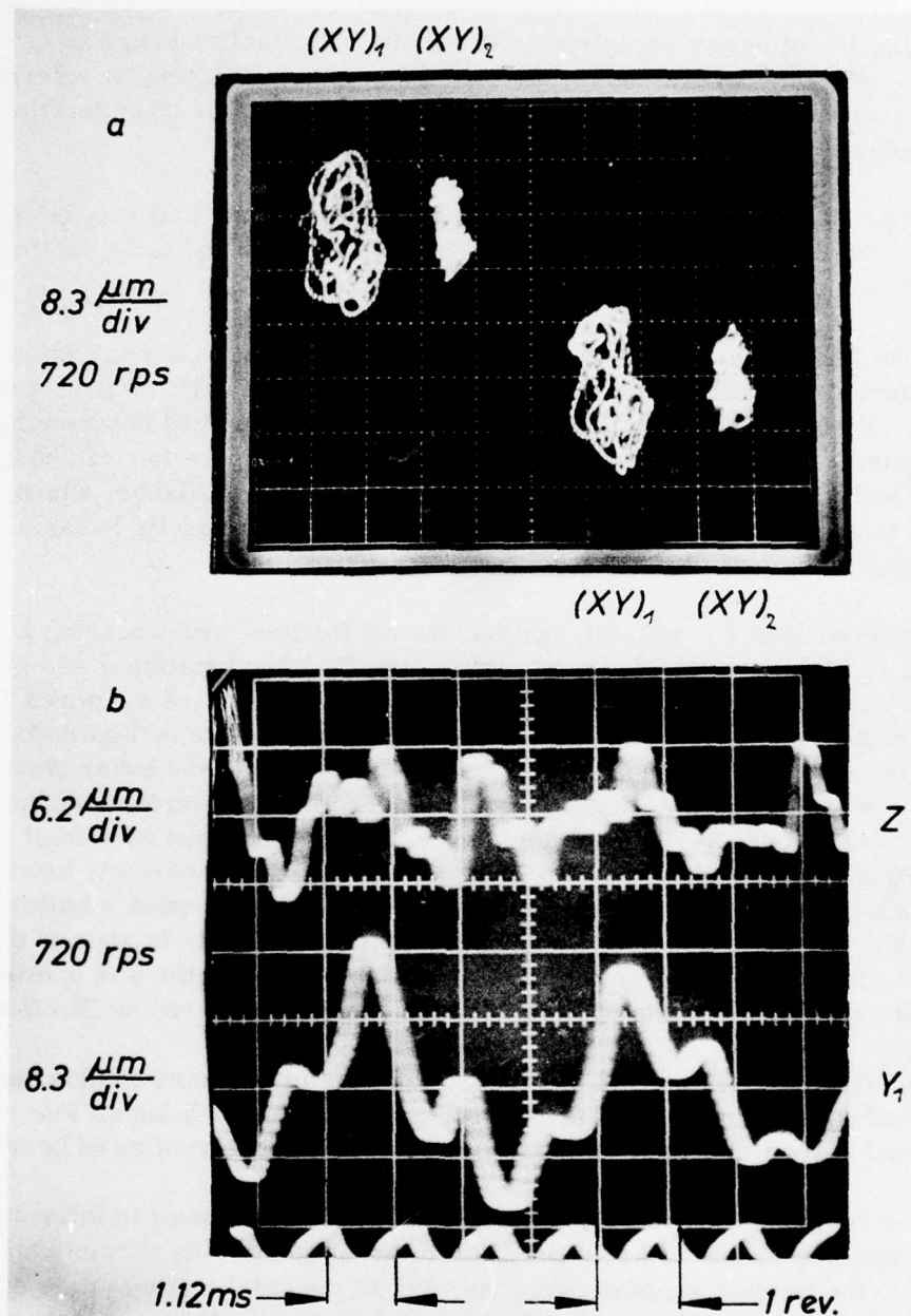
FIGURE 72. EFFECT OF THRUST LOAD AT N = 720 \text{ rps} ON MOTION OF ROTOR IN JOURNAL FOIL-BEARINGS LLF-1J (TWO Cu-Be FOILS PER BEARING, EACH L \times D \times t_f = 20 \times 30 \times 0.051 \text{ mm} . SIX TURNS, \bar{c} \approx 59 \mu\text{m} ). FLEXIBLE THRUST BEARING LLF-2T (INCONEL X-750 MEMBRANE, t_m = 215 \mu\text{m} . STEEL SPIDER SPRING, t_p = 170 \mu\text{m} ; \bar{t}_s = 53 \mu\text{m} ). (a) UPPER LEFT: TRAJECTORIES IN THE ABSENCE OF THRUST LOAD. LOWER RIGHT: TRAJECTORIES WITH THRUST LOAD F = 127.6 \text{ N} . (b) AXIAL MOTION OF RUNNER RELATIVE TO SUPPORT PLATE ( Z ) AND VERTICAL MOTION ( Y_1 ). THRUST LOAD F = 127.6 \text{ N}
