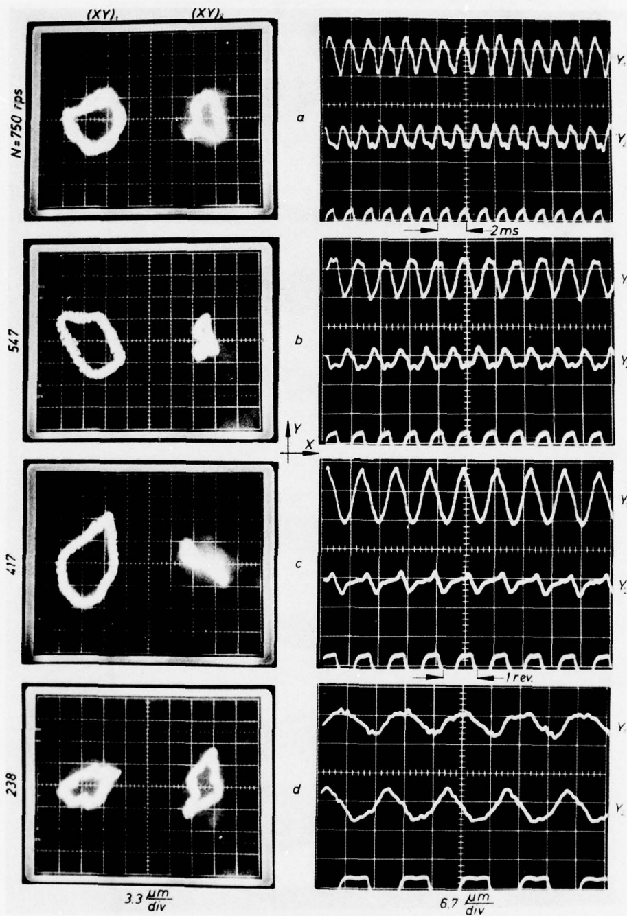
FIGURE 84. TRAJECTORIES AND TIME-BASE RECORDS OF MOTION IN (XY)_{1,2} AND (Y_1Y_2) PLANES WITH ASYMMETRIC UNBALANCE U_1 = 19.3 \mu\text{m. N} AND U_2 = 23.2 \mu\text{m. N} .-JOURNAL FOIL BEARING LLF-2J (OCTAGONALLY BENT BACKING AND 2-1/4 INNER TURNS. ONE STEEL FOIL PER BEARING, L \times D \times t_f = 20 \times 30 \times 0.054 mm. JOURNAL DIAMETER = 29.87 mm, FOIL-CARTRIDGE BORE = 30.61 mm).-FLEXIBLE THRUST BEARING UNLOADED.
