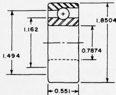
Figure 4. Basic 204 Size Test Bearing Geometry
