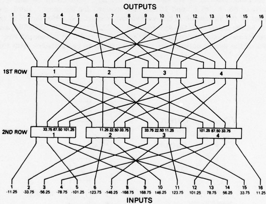
Fig. 2b —Sixteen-port Butler matrix
