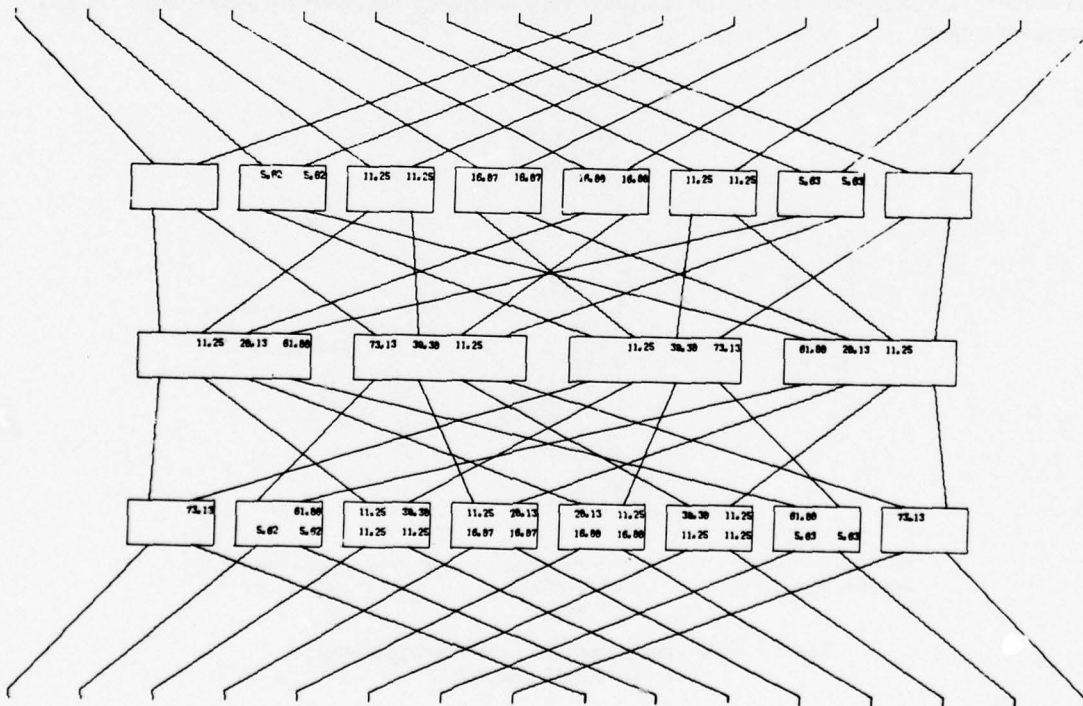
Fig. 6c —Symmetric 16-port matrix using one row of 4-port and two rows of 2-port building blocks
