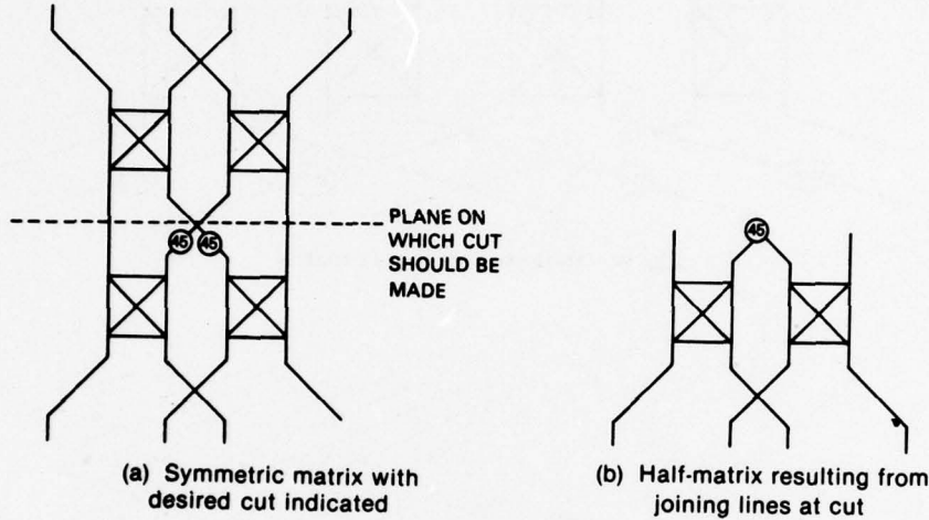
Fig. 8 - Half four-port matrix illustrating method of making cut
