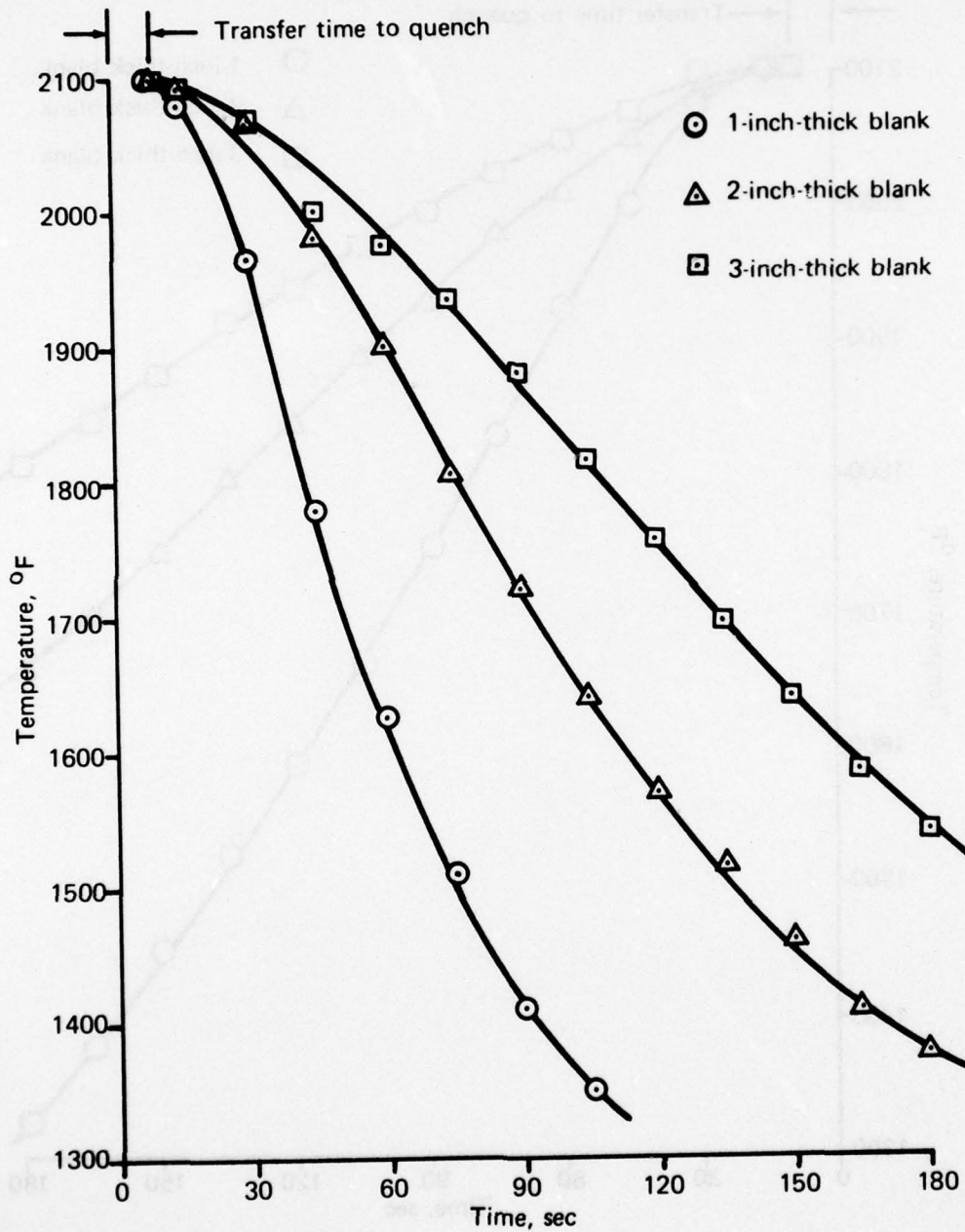
(b) 1200°F salt quench
