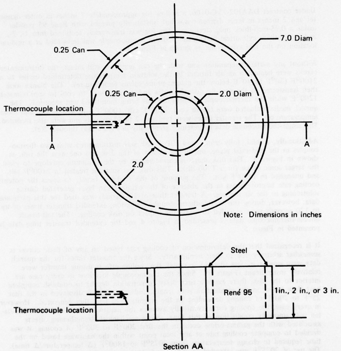
Figure 1. Cylindrical cooling blank configuration and thermocouple location.
