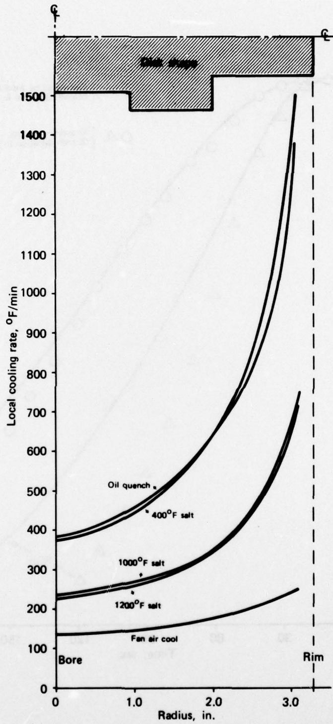
Figure 15. Disk local cooling rate variation for each quench media.
