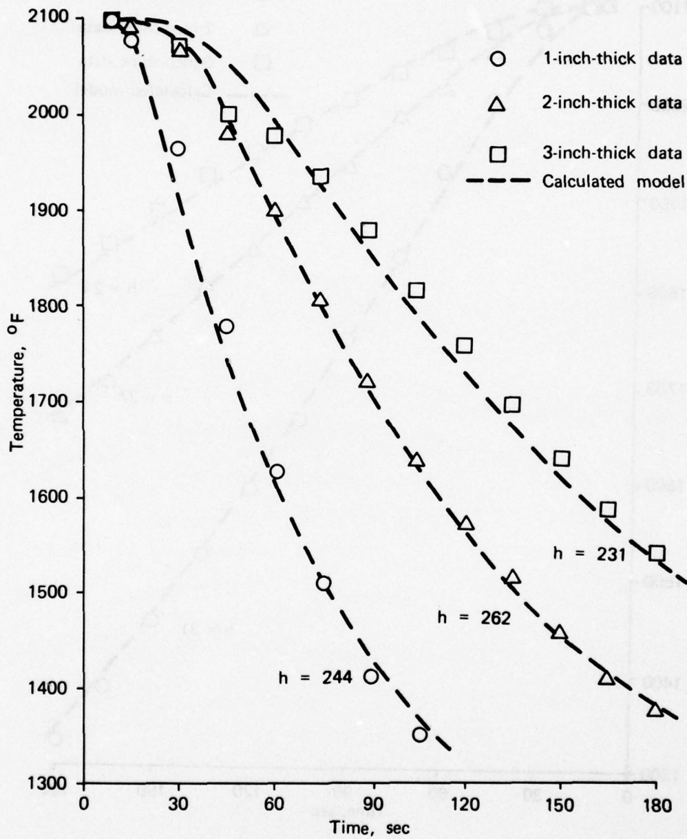
(b) 1200°F salt quench
