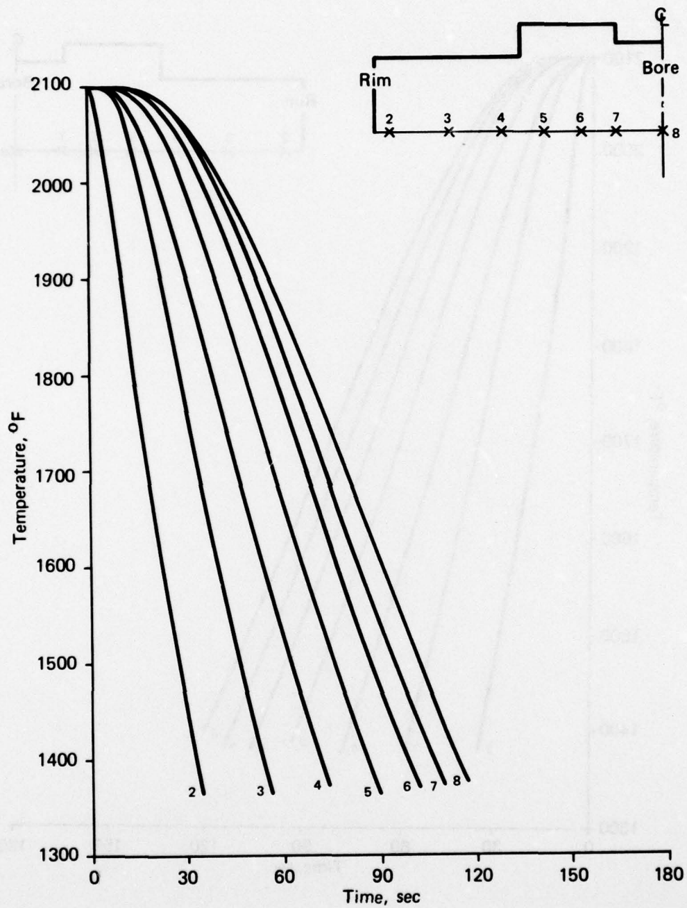
(e) Oil quench
