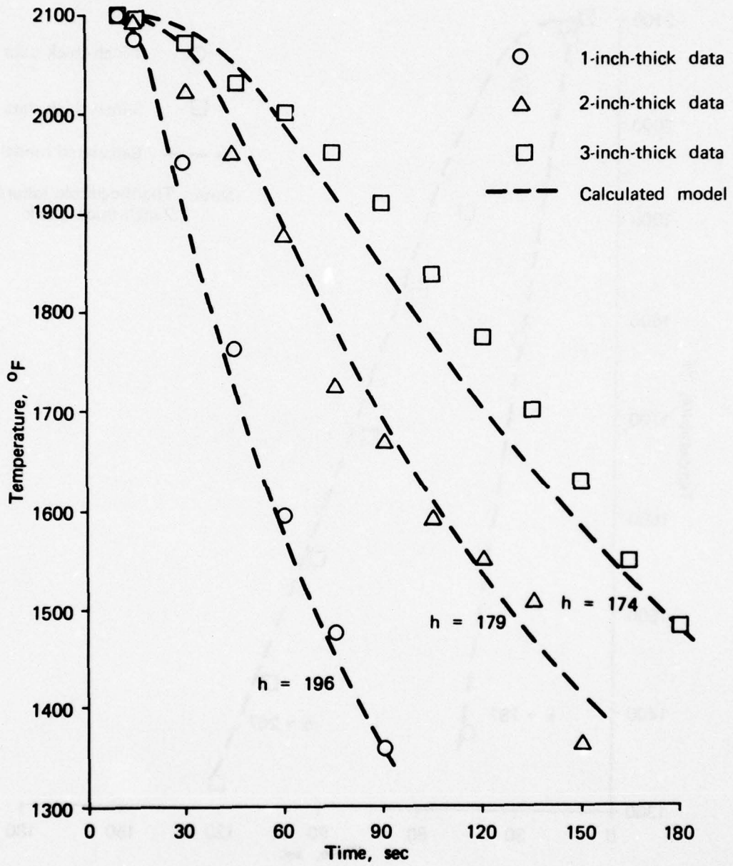
(c) 1000°F salt quench
