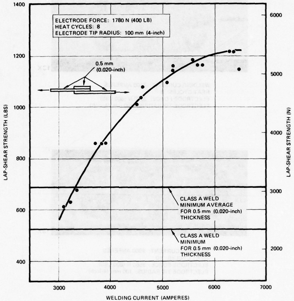
FIGURE 14. EFFECT OF WELDING CURRENT ON SPOT WELD PROPERTIES FOR Ti-6Al-4V, 0.5/0.5/0.5 mm (0.020/0.020/0.020-inch)
