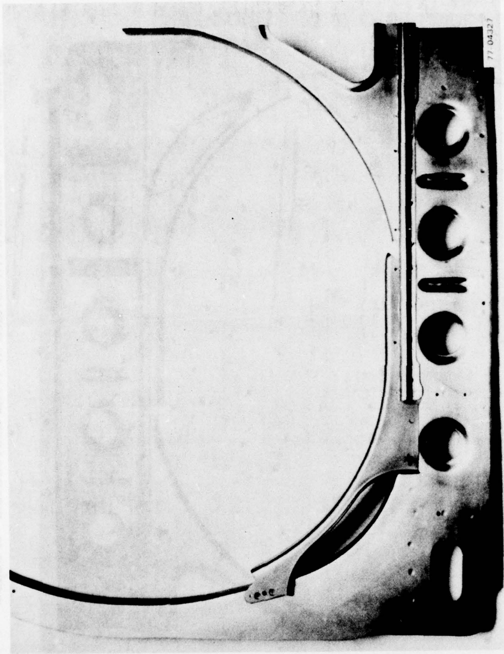
FIGURE 41. WELDBRAZED TI-6Al-4V FORMER HALF SECTION - FRONT SURFACE
