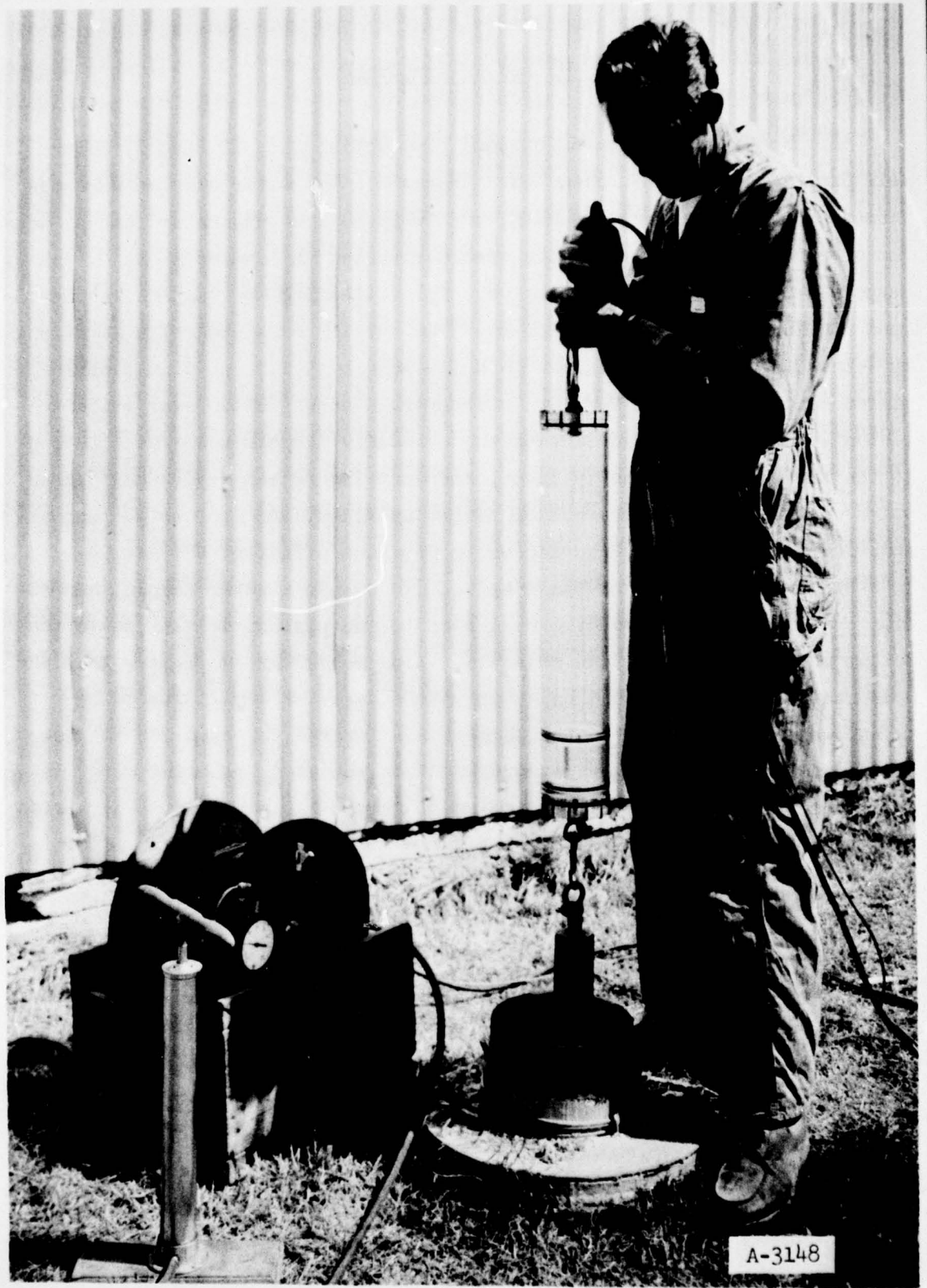
Fig. B1. WES-designed water sampler
