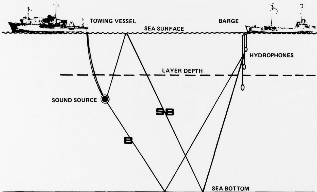
FIG. 1 EXPERIMENTAL ARRANGEMENT
