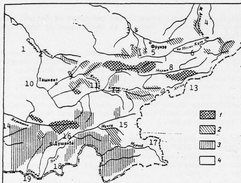
Figure 2. Map of the predominant processes of transformation of the snow layer through the territory of Central Asia in the 1959 - 1970 period. 1 - regions with predominant development of a snow layer of the disintegration type; 2 - regions with an unstable developmental character of the snow layer; 3 - regions with predominant development of a snow layer according to the packing type; 4 - regions where processes of transformation of the snow layer have not been studied.
