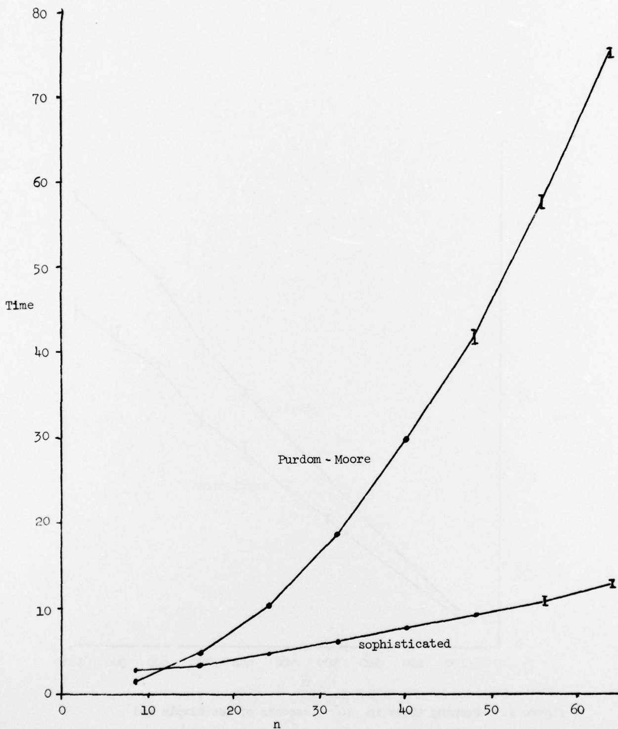
Figure 7. Running times in 10^{-3} seconds of the Purdom-Moore algorithm and the sophisticated version of the fast algorithm.
