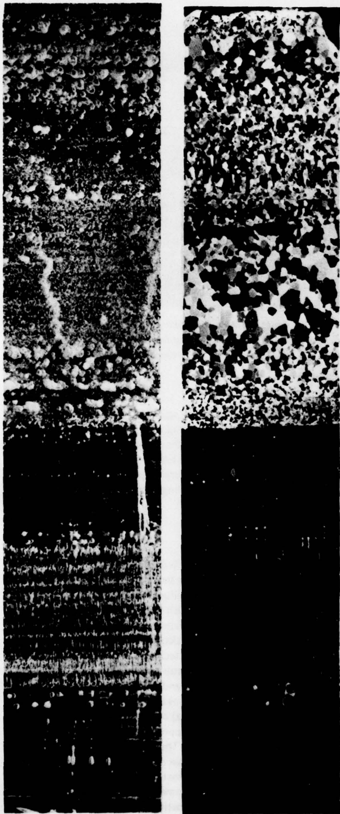
Figure 2. Vertical sections illustrating stratigraphic (a) and structural (b) characteristics of a lake ice sheet, Canaan Street Lake, New Hampshire. Transition from snow-ice to lake ice is especially well marked. In this instance, the lake ice is composed entirely of crystals with vertical c-axes. Ice thickness is 43 cm.
