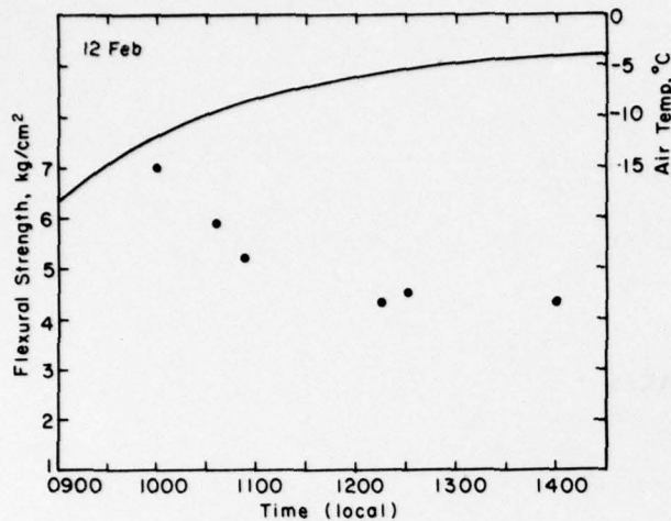
a. Variation of flexural strength with temperature.
