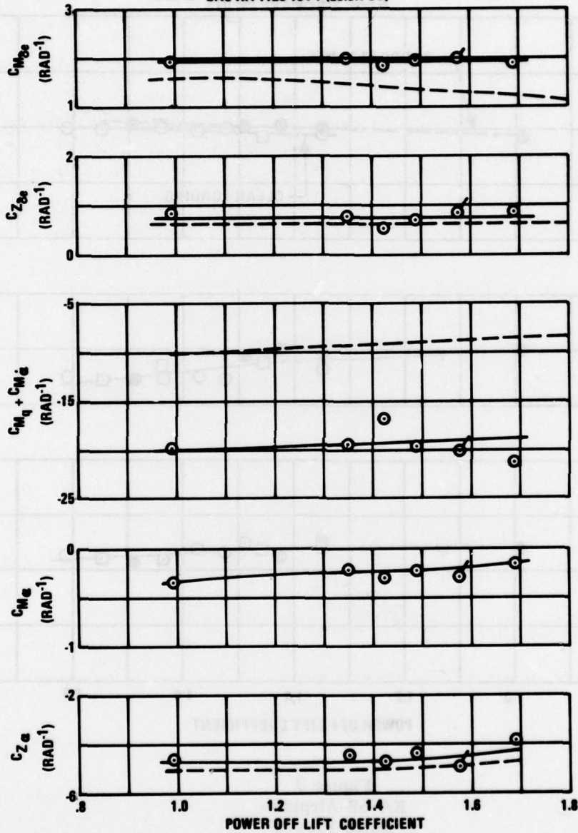
Figure 2 EA-6B Airplane BuNo 156478 Short Period Aerodynamic Coefficients
