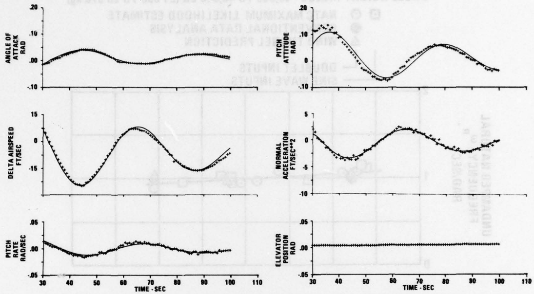
Figure 6 EA-6B Airplane BuNo 156478 Time History Comparison of Long Period Characteristics
