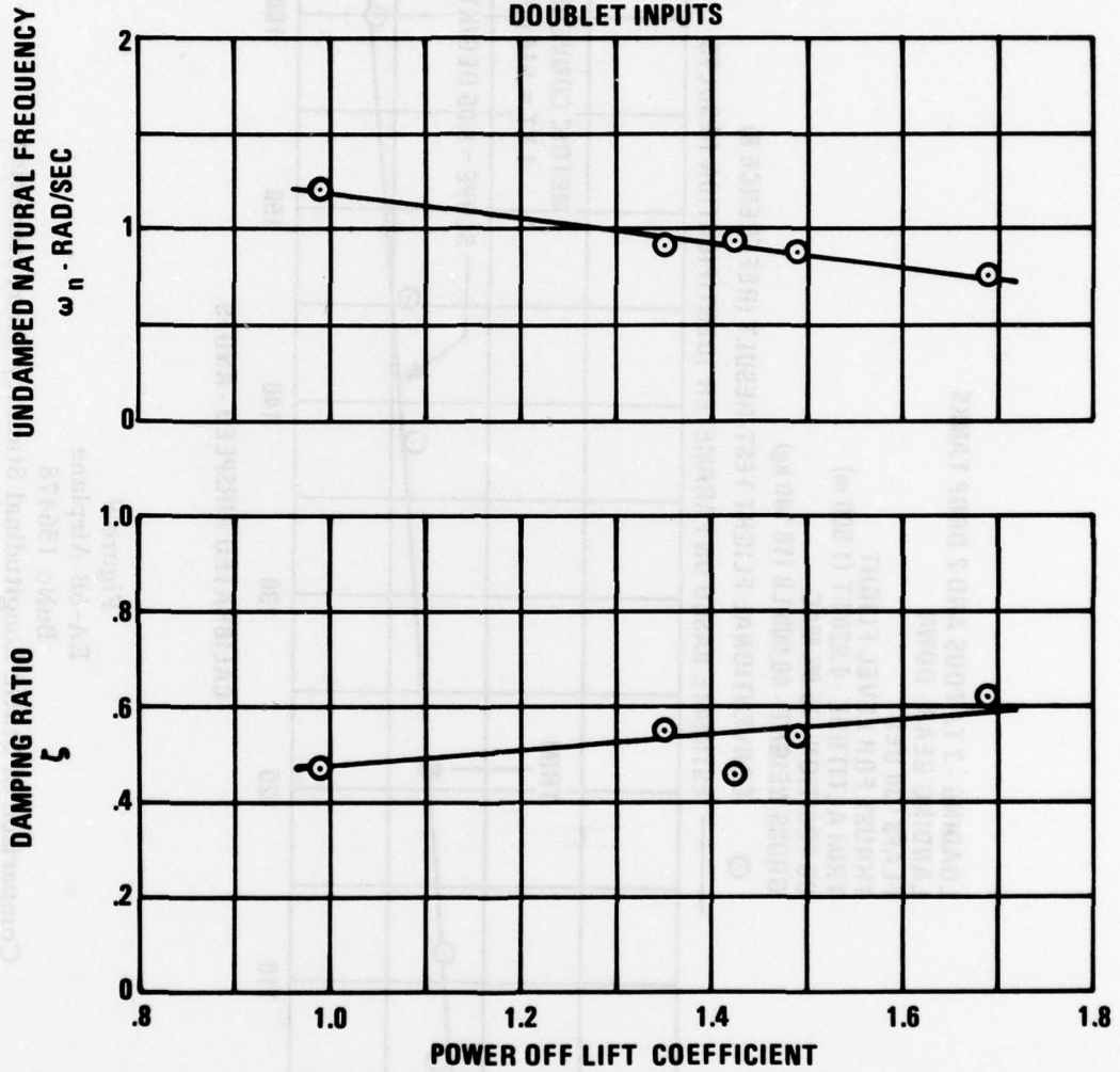
Figure 8 EA-6B Airplane Short Period Frequency and Damping Characteristics
