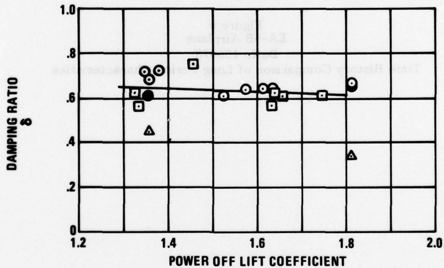
Figure 7 EA-6B Airplane BuNo 156478 Short Period Frequency and Damping Characteristics
