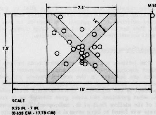
Figure 3 TOW Missile Impacts Combined Targets
