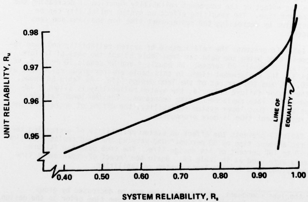
Figure E11. Relationship between system and unit reliability.
