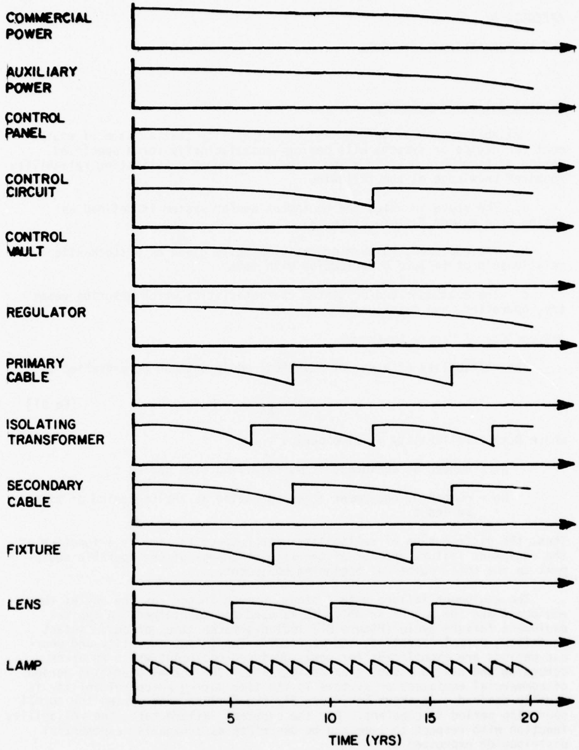
Figure A9. Component operation curves.
