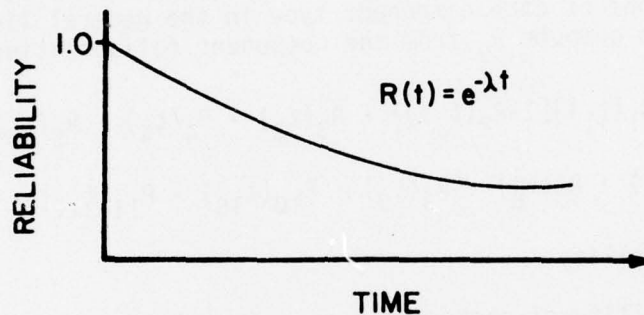
Figure 2. Reliability distribution.
