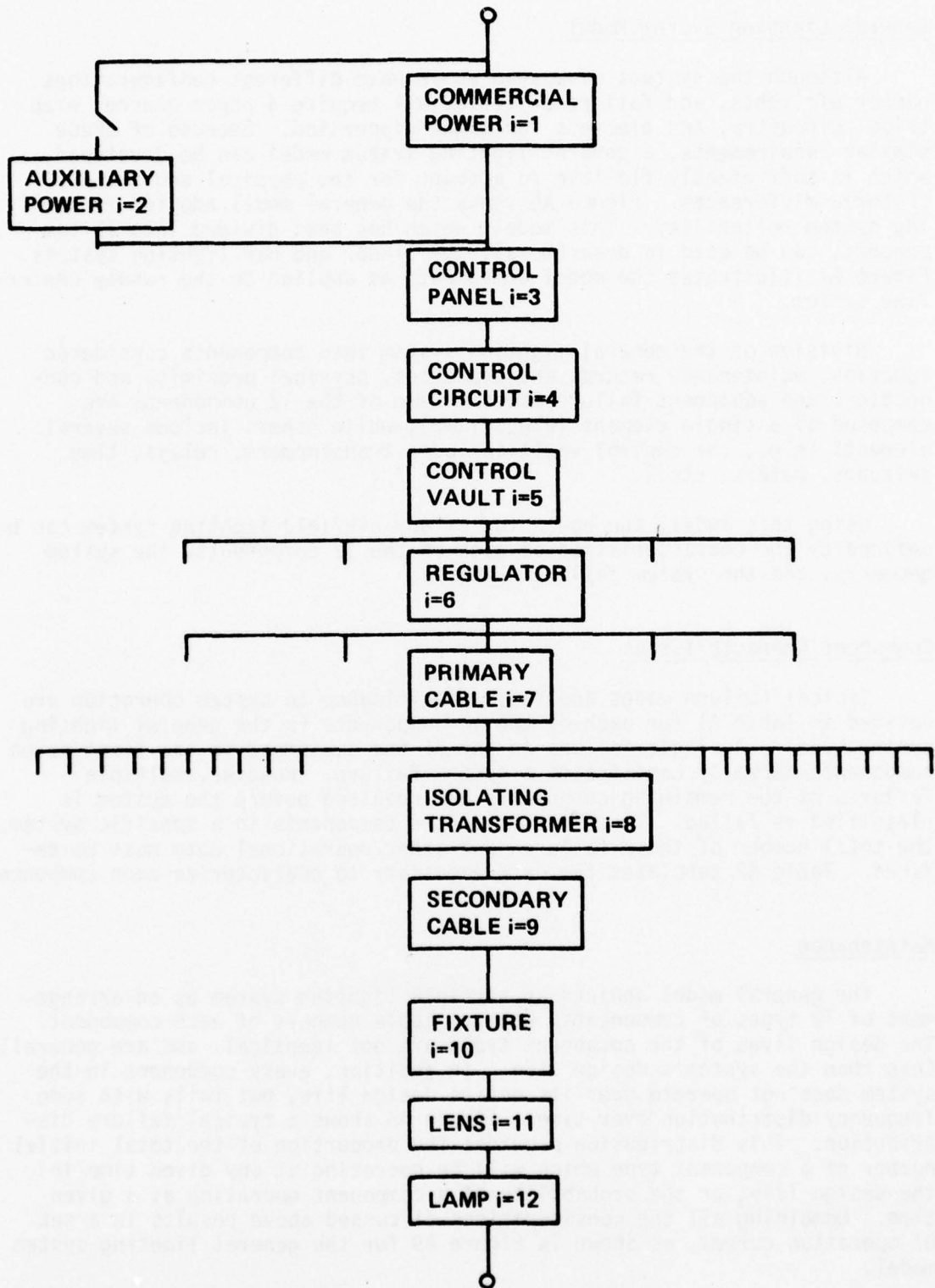
Figure A6. General lighting system model.
