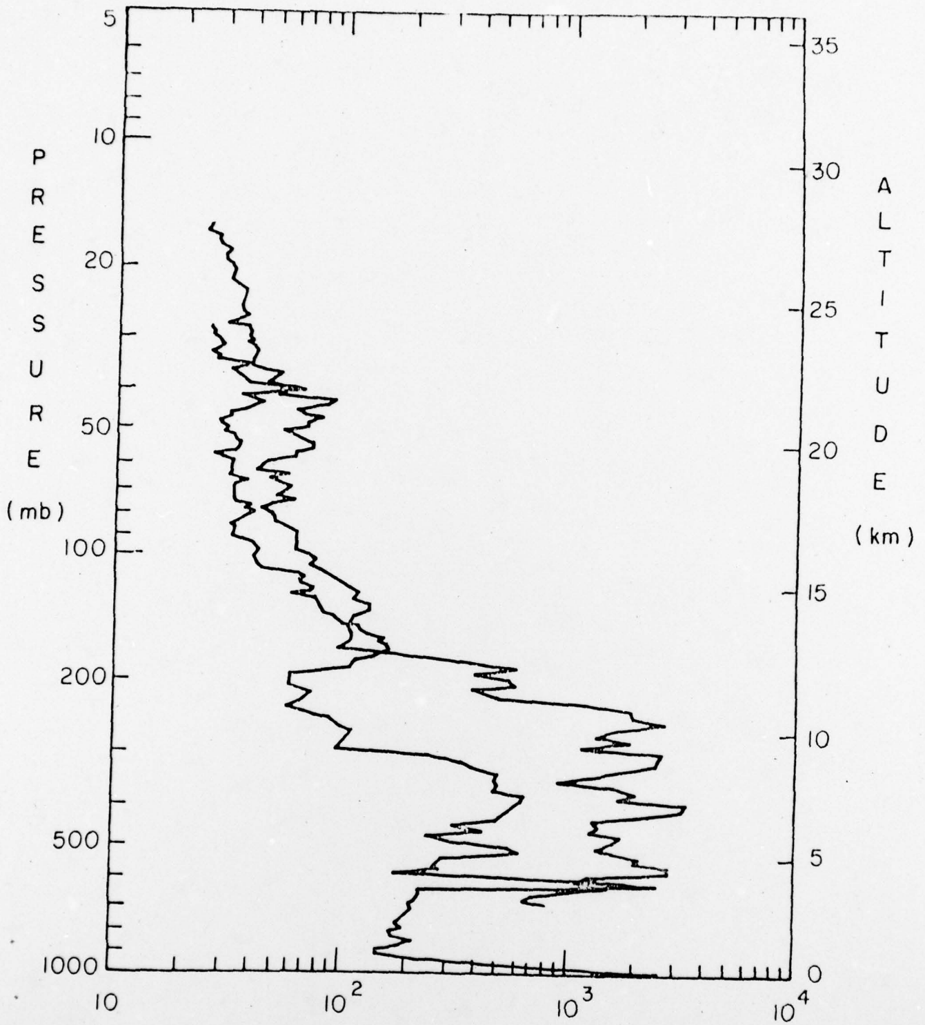
Figure 5. A comparison of the McMurdo, Antarctica sounding and the South Pole sounding. The South Pole sounding has higher values in the troposphere.
