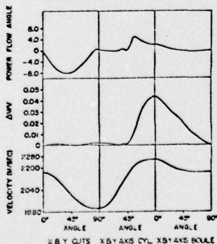
Figure 1. The variation of the SAW velocity, \Delta v/v and the power flow angle for standard crystallographic cuts in \text{LiIO}_3 . Z cut occurs at X and Y axis cylinder, 0°. Z-axis boule at X and Y cut, 90° and Z-axis cylinder at X and Y-axis boule, 90°.
