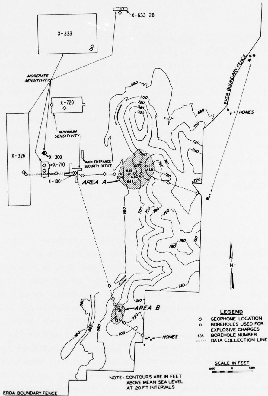
Figure 1. Location plan
