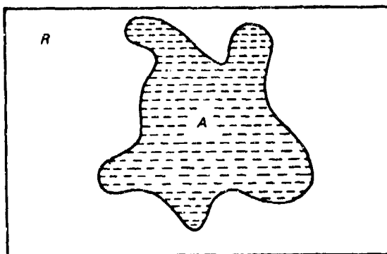
FIGURE 3.3. LAKE OF AREA A ENCLOSED IN RECTANGLE OF AREA R. FROM REFERENCE [10].
