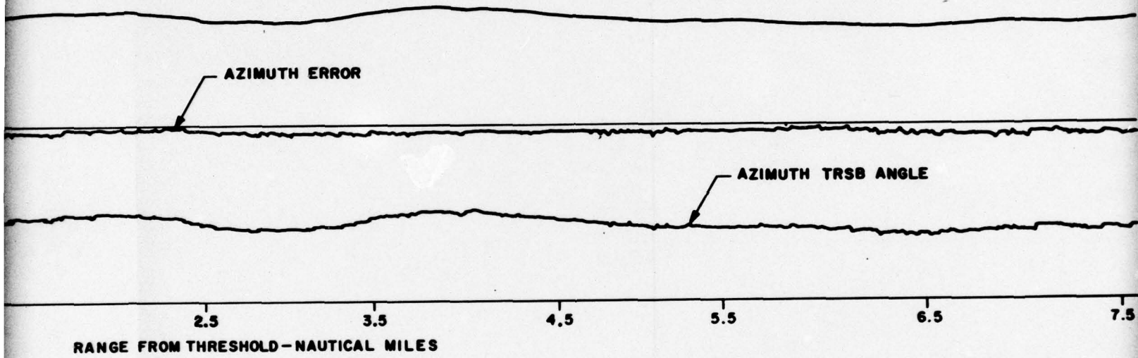
FIGURE 15. SAMPLE AZIMUTH STRIP CHART RECORDING FOR 11-24-77
