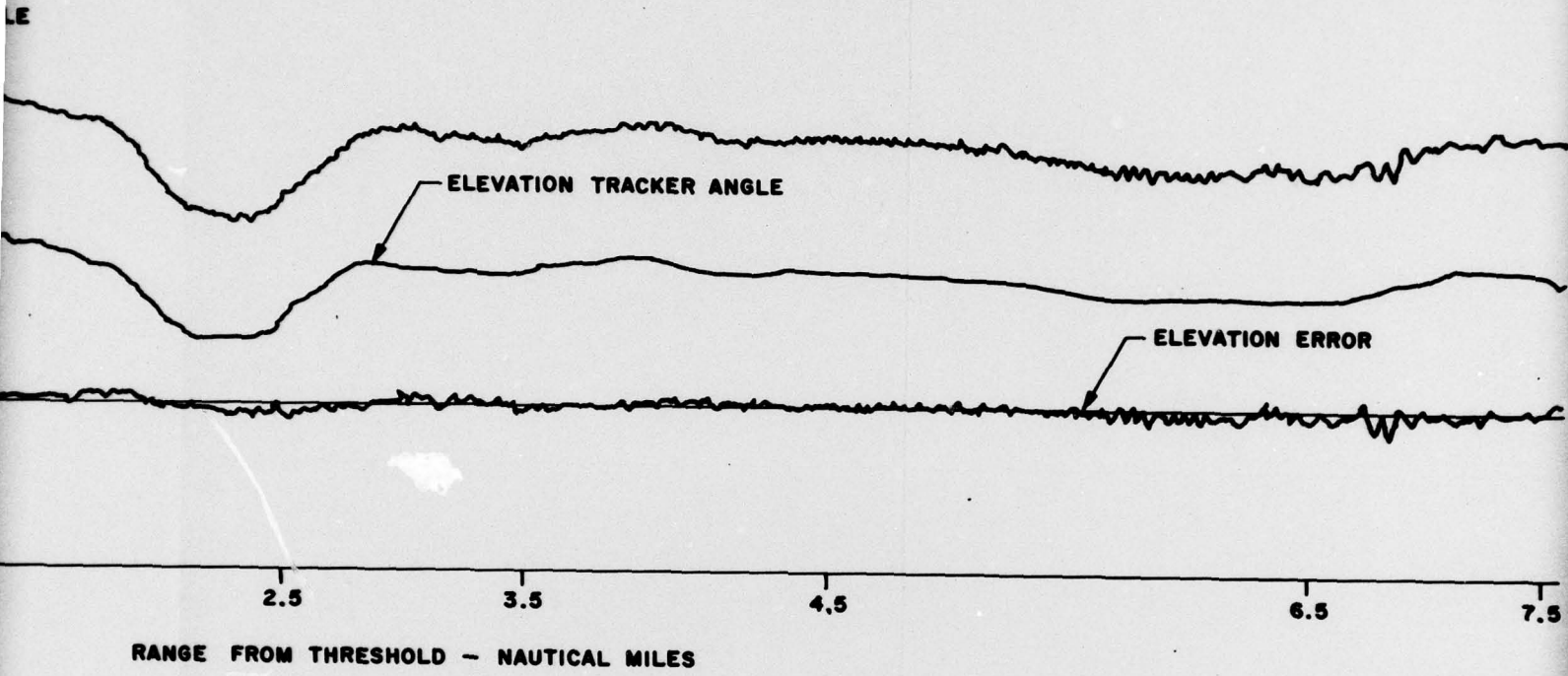
FIGURE 18. SAMPLE ELEVATION STRIP CHART RECORDING FOR 11-25-77
