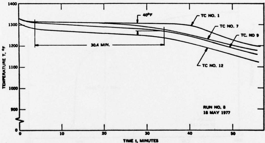
Figure 69. Measured Temperatures During Discharge of Thermal Energy Storage Unit (Power Extracted at Hot Cylinder P = 326 \text{ watt} )
