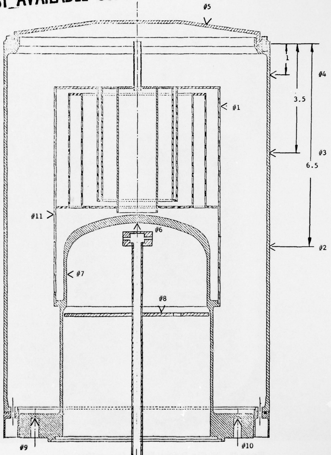
Figure 39. Thermocouple Locations for Testing of Hi-Cap Thermal Energy Storage Unit in Its Final Configuration
