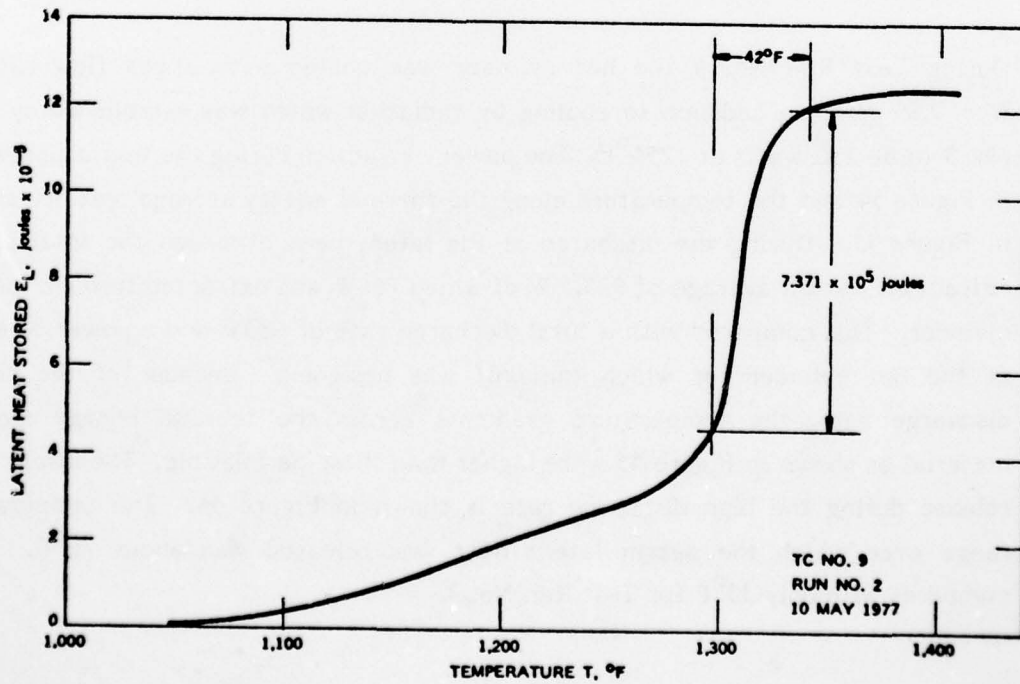
Figure 48. Latent Heat Storage in Thermal Energy Storage Material During Charging (Heater Power P_{in} = 393.67 \text{ watt} )
