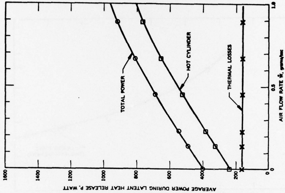
Figure 71. Average Power During Discharge of Thermal Energy Storage Unit (E = 7.173 x 10 5 joules)
