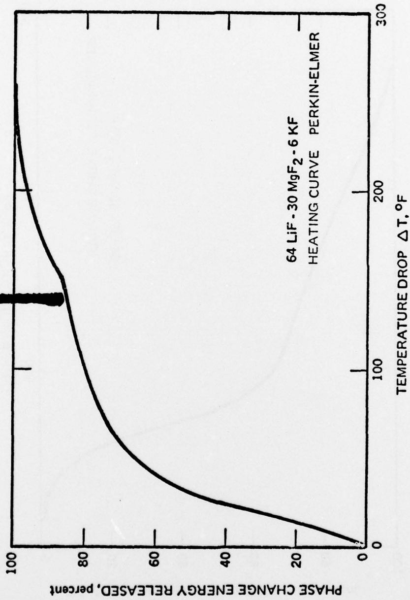
Figure A-7. Relative Energy Extraction from Thermal Energy Storage Material (Starting Temperature 1328°F)
