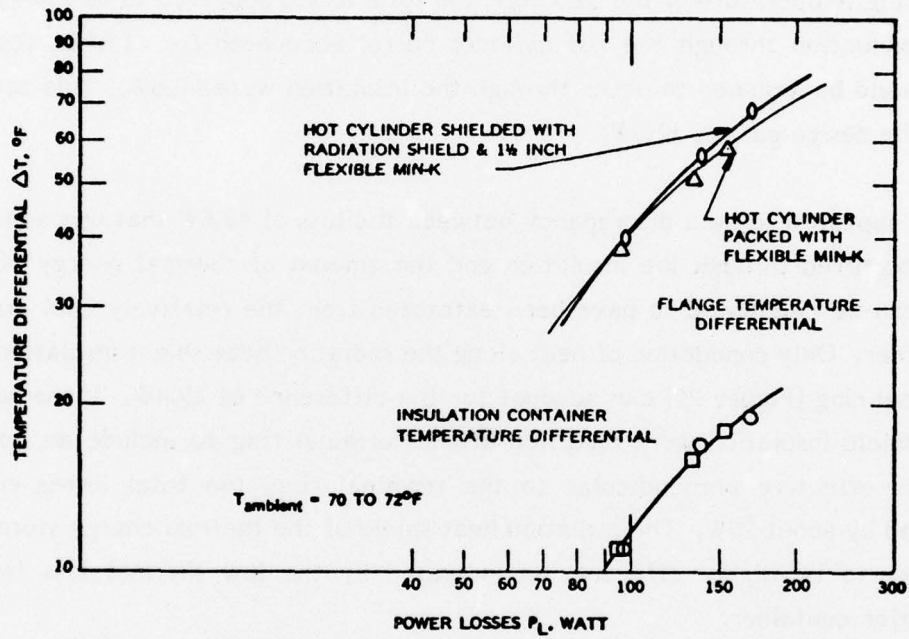
Figure 74. Terminal Ring and Insulation Container Temperature Differential at Steady State Power Losses (Temperature Differential \Delta T = T - T_{ambient} )
