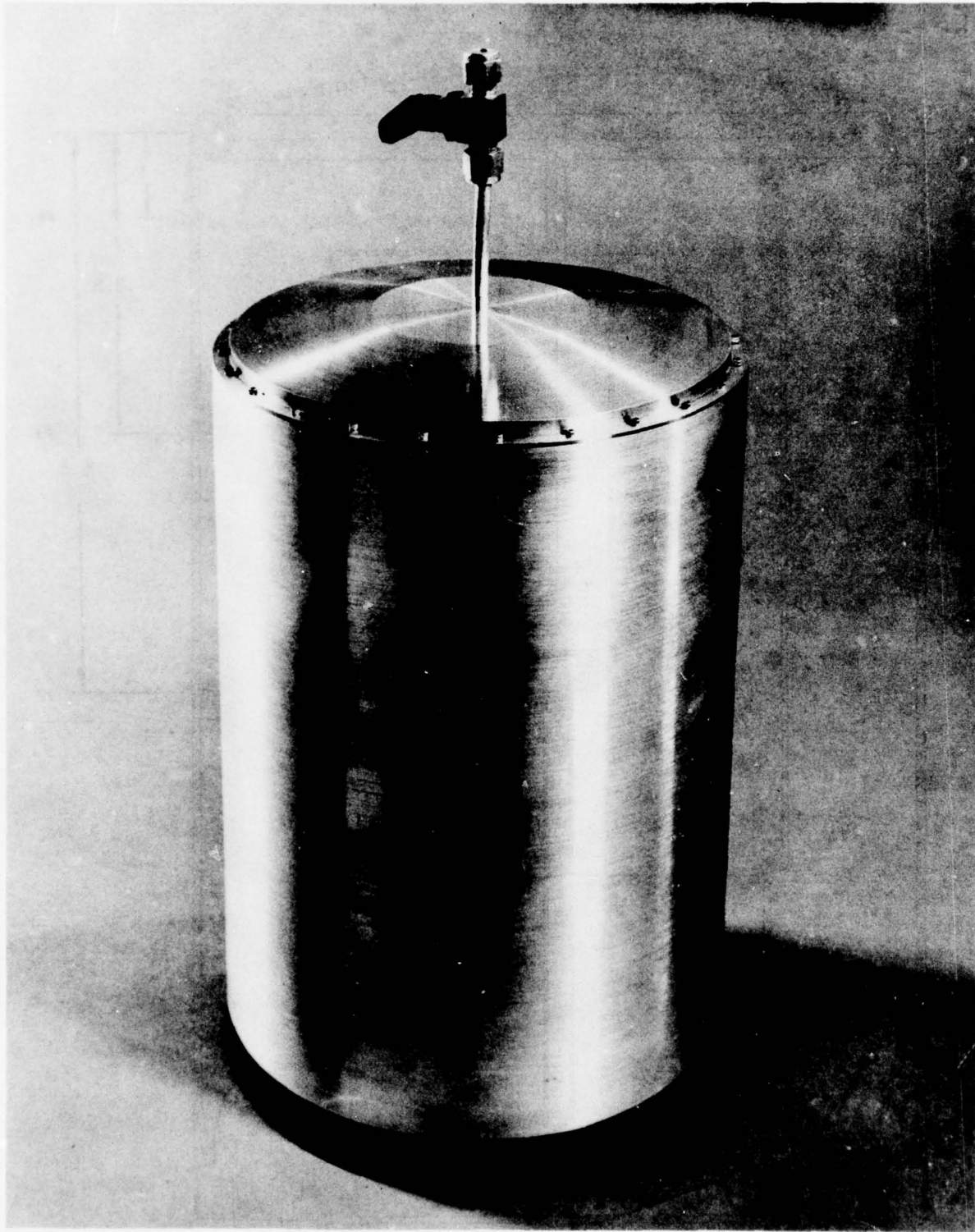
Figure 38. Hi-Cap Thermal Energy Storage Unit
