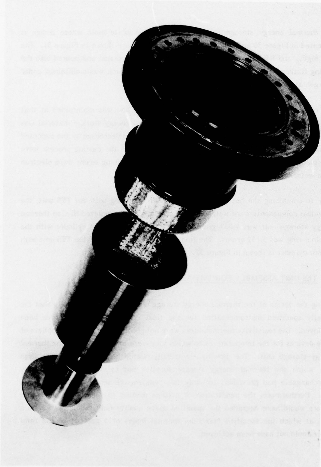
Figure 29. Thermal Energy Storage Unit with Hot Cylinder of Hi-Cap Vuilleumier Cooler Prior to Final Assembly and Loading with Thermal Energy Storage Material
