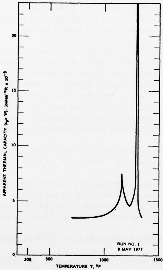
Figure 46. Apparent Thermal Capacity of Hi-Cap TES Unit
