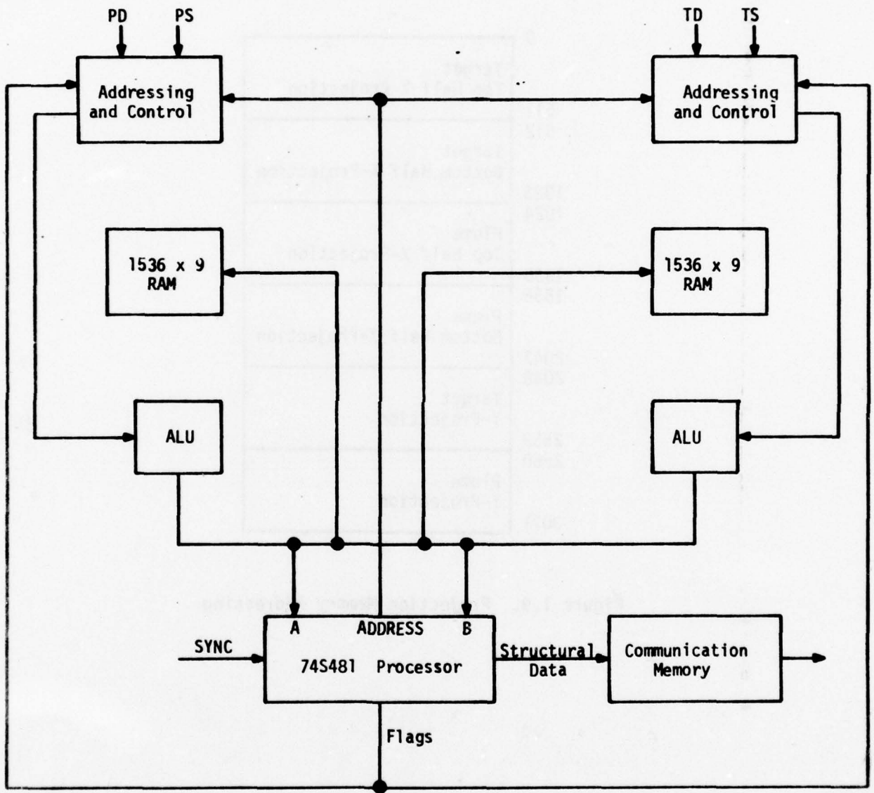
Figure 1.8. Projection Processor
