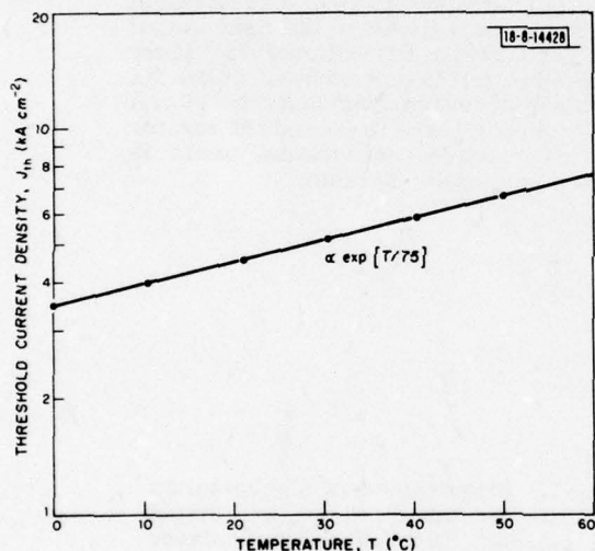
Fig. I-3. Threshold current density vs heat-sink temperature for a DH GaInAsP/InP laser emitting at 1.22 \mu\text{m} .
