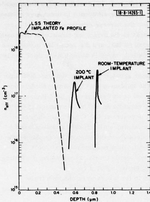
Fig. III-4. Effective carrier concentration vs depth obtained from capacitance-voltage measurements for two InP ( n = 6 \times 10^{16} cm -3 ) samples after a multi-energy Fe + implant and a 725°C 15-min. anneal. One sample was implanted at room temperature and the other at 200°C.
