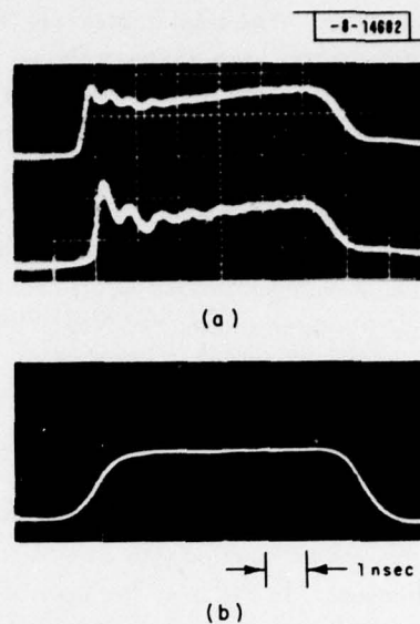
Fig.1-6. Response (a) of a germanium avalanche photodiode to the light output of a DH 1.22- \mu m DH GaInAsP/InP laser driven by the 50-mA current pulse (b). DC bias current through laser is 300 mA for the upper trace in (a) and 285 mA for the lower trace. Horizontal scale is 1 nsec per major division.
