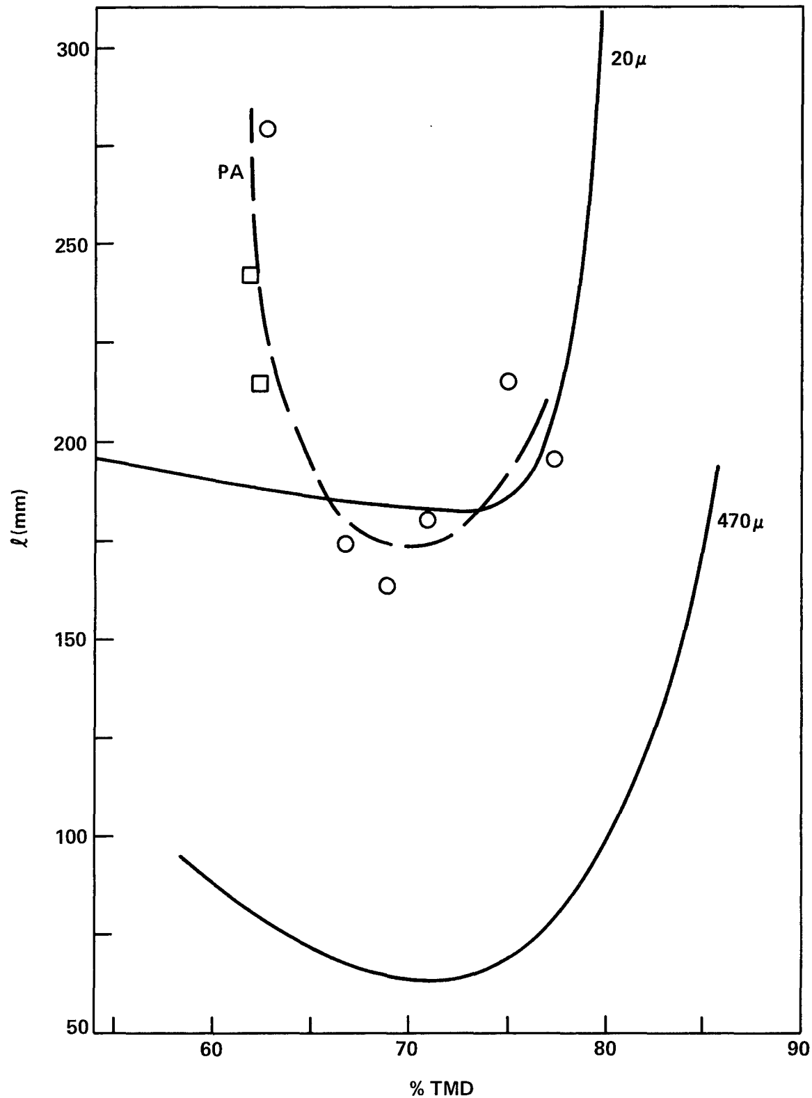
FIGURE 5 VARIATION OF PREDETONTATION COLUMN LENGTH WITH POROSITY OF PICRIC ACID COMPARED TO THAT OF FINE AND COARSE TETRYL
