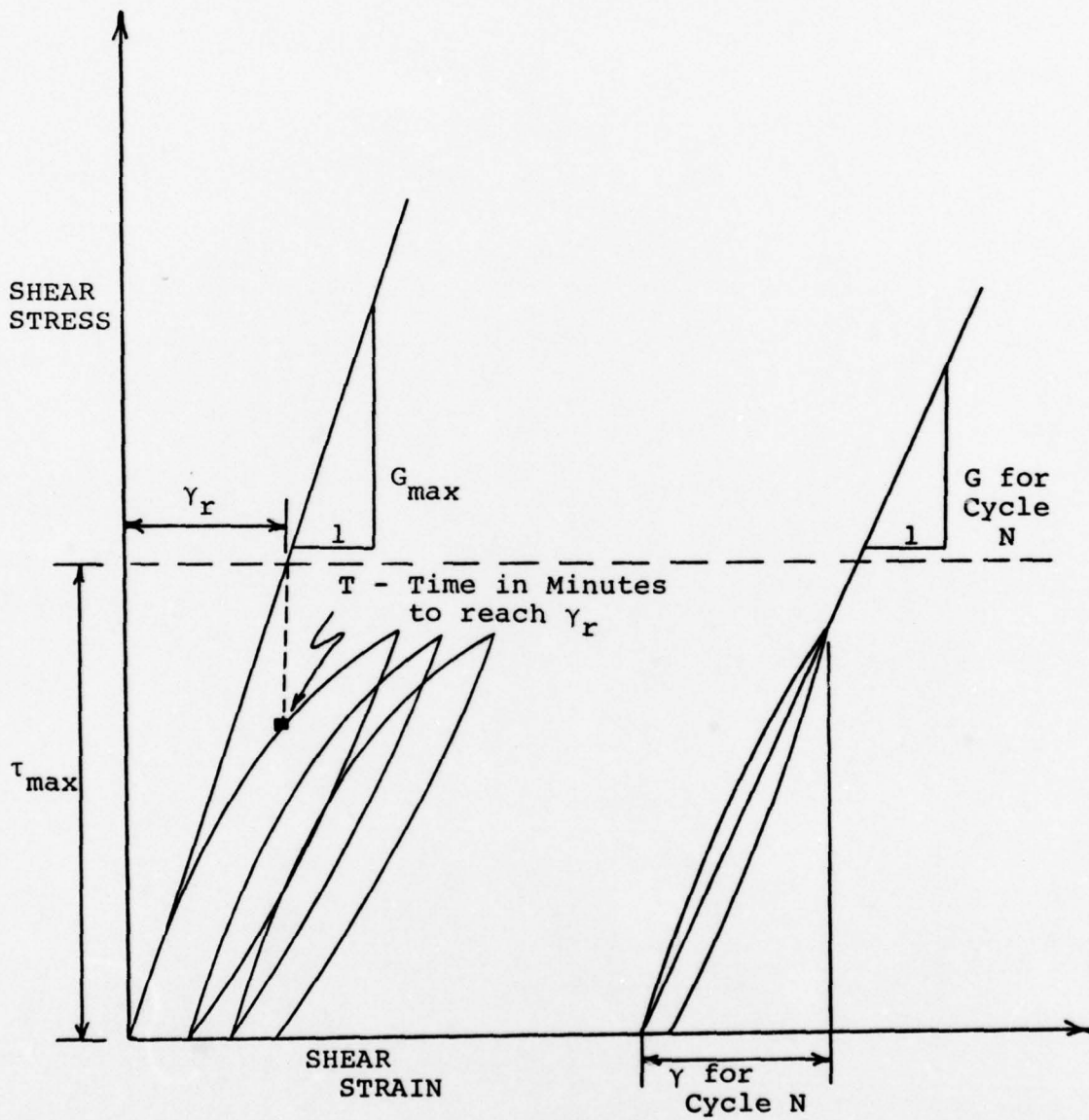
FIGURE 2 SCHEMATIC OF SHEAR STRESS-SHEAR STRAIN RELATION (From Reference 1).
