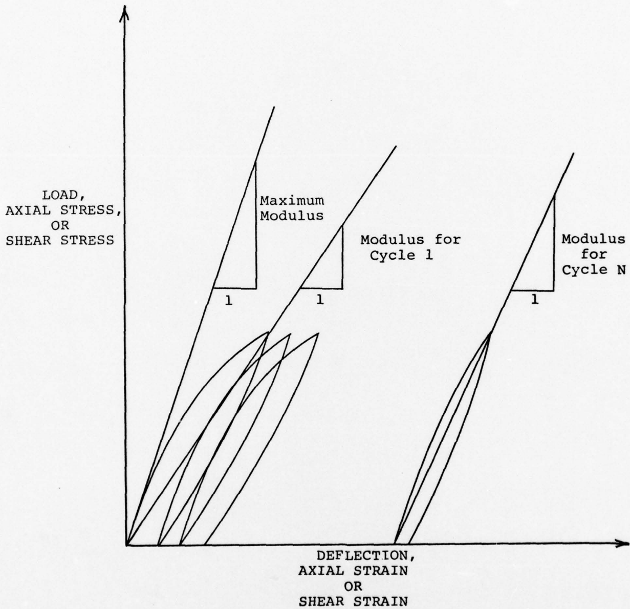
FIGURE 1 SCHEMATIC OF LOAD-DEFLECTION, AXIAL STRESS- AXIAL STRAIN, OR SHEAR STRESS-SHEAR STRAIN RELATIONSHIP FOR SOIL.
