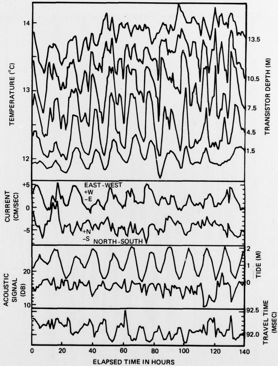
Figure 3. Smoothed time series (from top to bottom) for temperature, current, surface tide, acoustic signal, and travel time. For the current time series +W means that the current is toward the west, -E toward the east, +N toward the north and -S toward the south.
