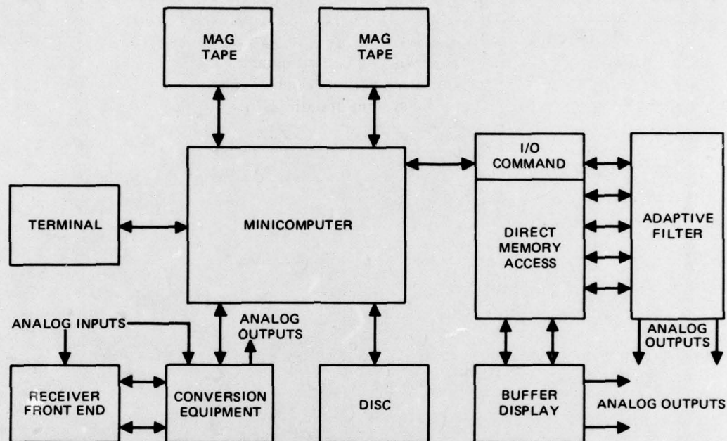
Figure 2. Test-bed component interconnections.
