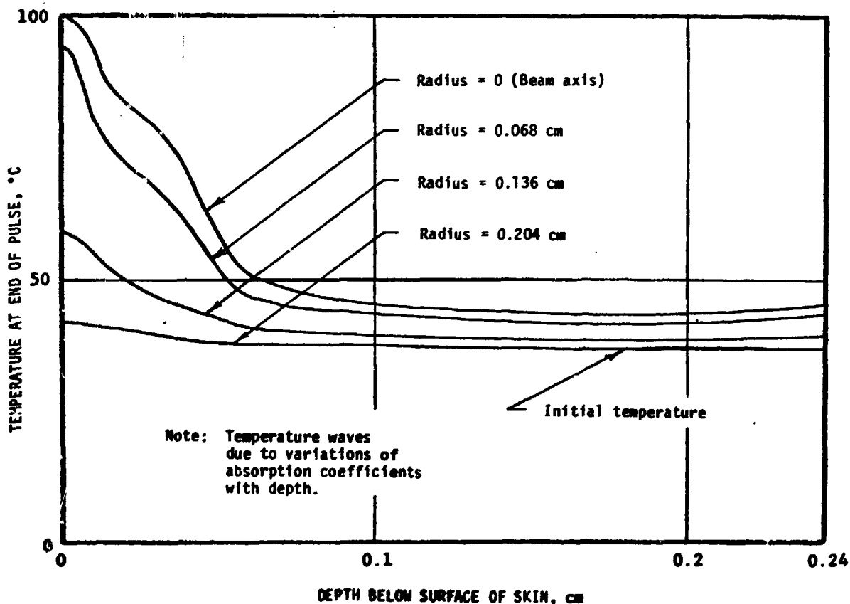
Figure 18. Temperature predictions due to ruby laser pulse (pulse energy = 1.74 joules, pulse duration = 5 \cdot 10^{-4} sec; beam radius = 0.17 cm at 1/e^2 points).
