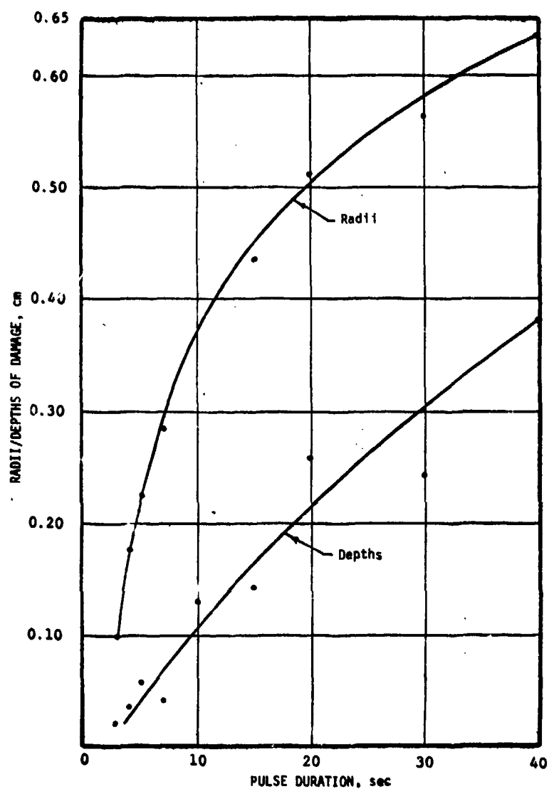
Figure 15. Radii and depths of damage produced by CO 2 laser (1.53 watts, beam radius at 1/e 2 point = 0.710 cm).
