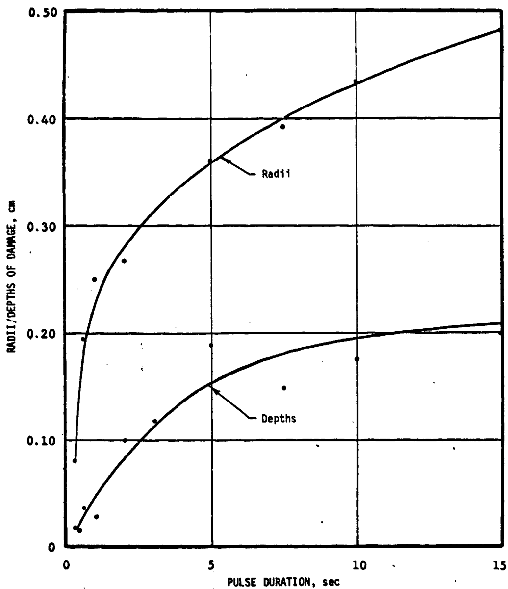
Figure 16. Radii and depths of damage produced by CO 2 laser (1.97 watts, beam radius at 1/e 2 point = 0.383 cm).
