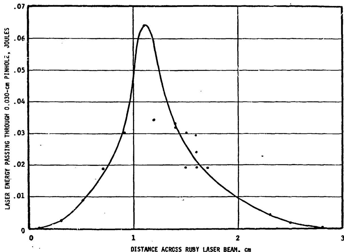
Figure 14. Profile of normal ruby laser beam. Curve is "eyeball" fit to the data.
