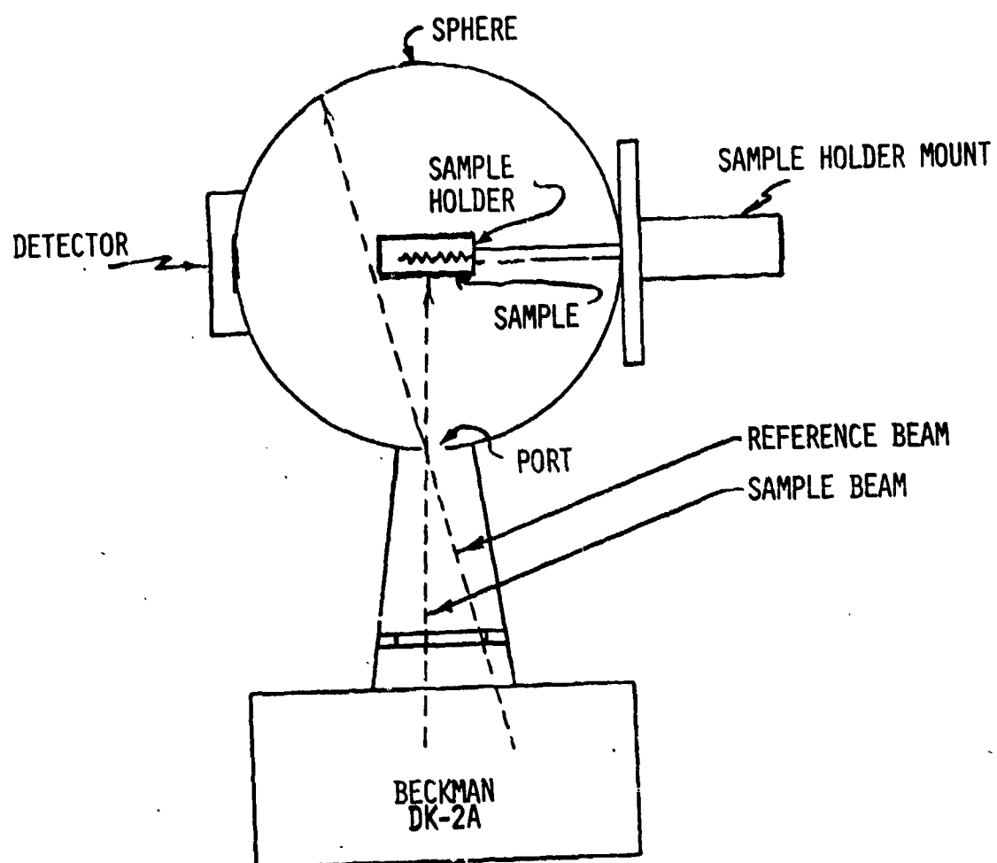
Figure 1. Schematic of integrating-sphere reflectometer.
