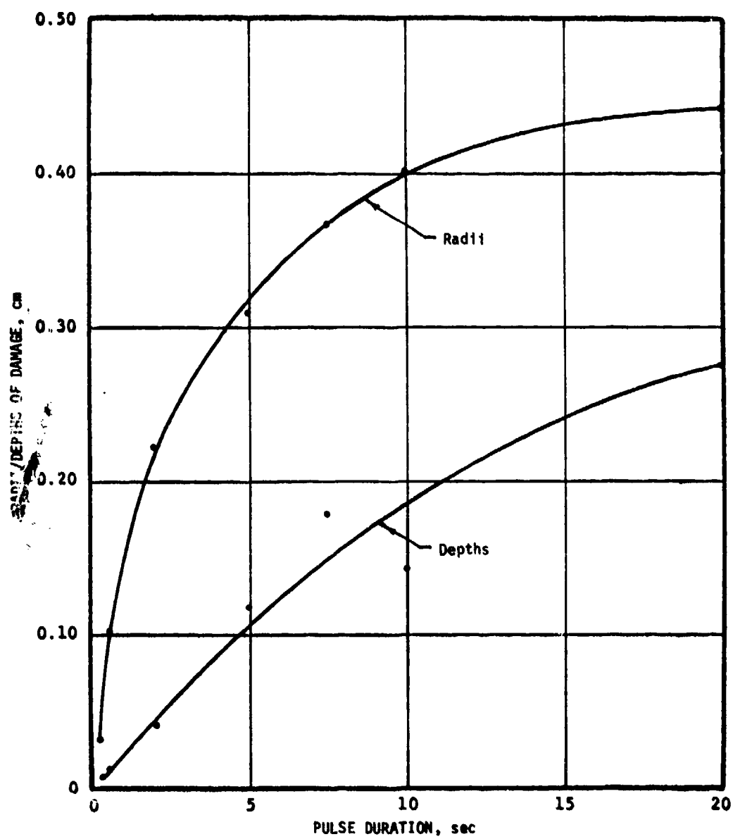
Figure 17. Radii and depths of damage produced by CO 2 laser (1.55 watts, beam radius at 1/e 2 point = 0.383 cm).
