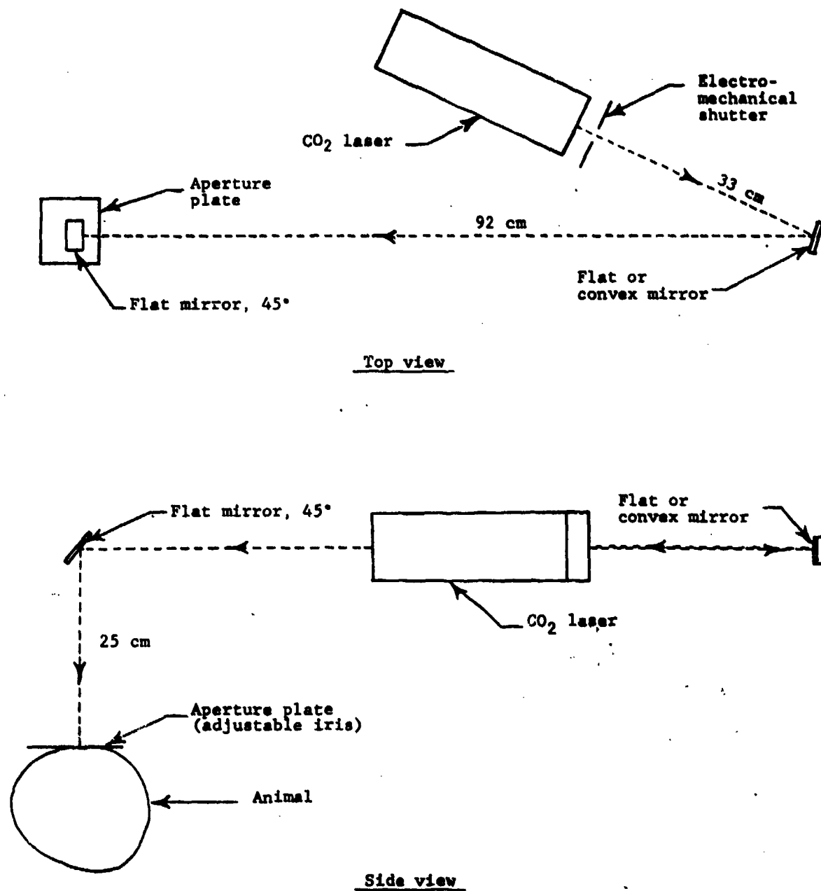
Figure 10. Optical system for controlling animal exposure (CO 2 laser).
