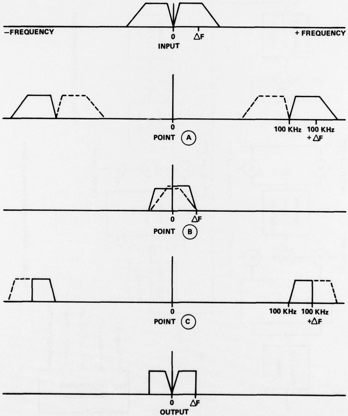
FIGURE 2. SYSTEM FREQUENCY SPECTRA, LOW-PASS MODE
