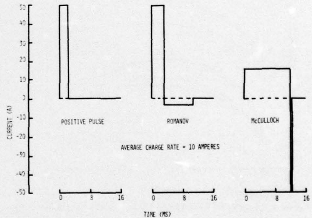
Figure 1. Pulse Charge Mode Wave Forms.
