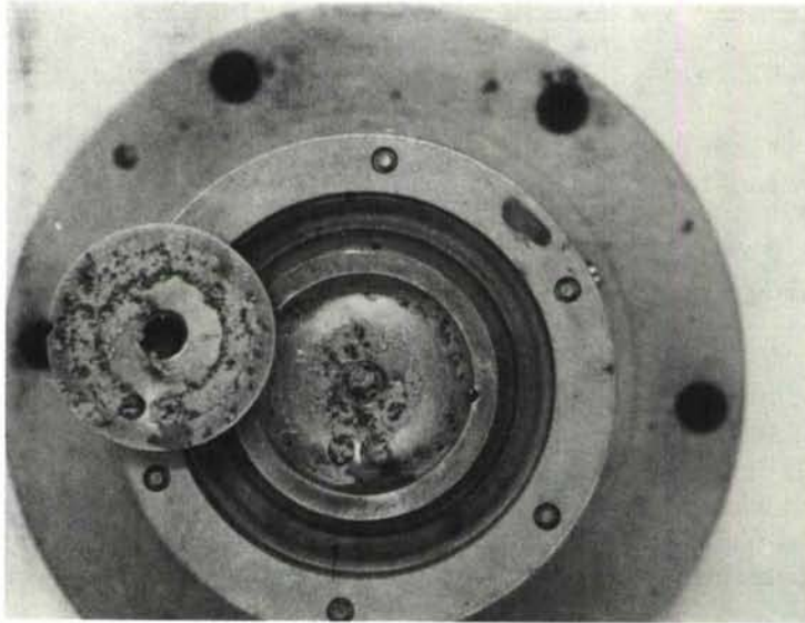
Figure 40 DC FCS 210 (OH term) Sealant After 1 Cycle (177 to -54°C) Plus Heat Portion of 2nd Cycle Upper Channel, Formulation #23
