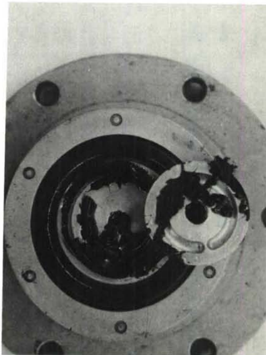
Figure 29 DC FCS 210/LS, 1:2 Copolymer Sealant With Fluoro- silicone Vulcanized Particles After 3 Cycles (177 to -54°C), Formulation #17
