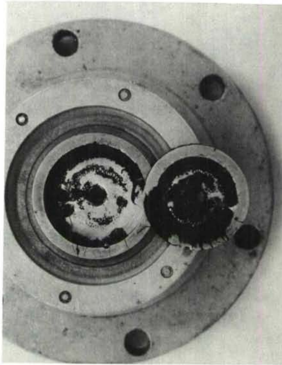
Figure 28 DC FCS 210/LS, 1:2 Copolymer Sealant With Beads After 1 Cycle (177 to -54°C), Upper Channel, Formulation #16
