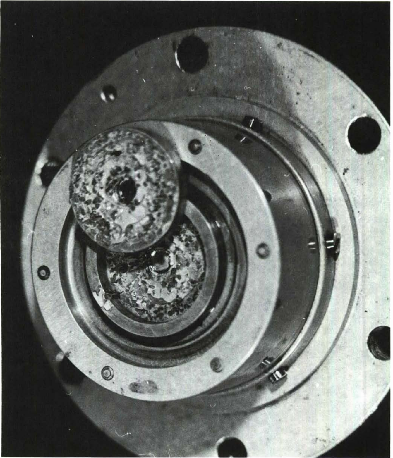
Figure 43 PNF 200 Sealant After 20 Cycles (177 to -54°C) Upper Channel, Formulation #26
