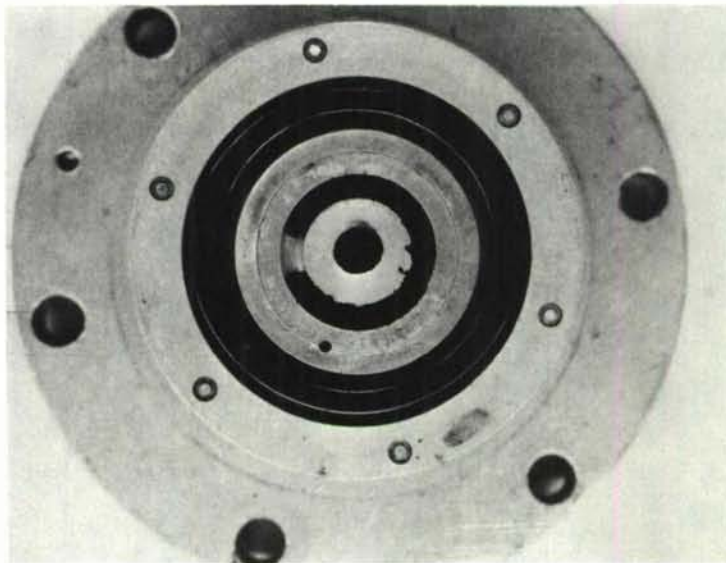
Figure 41 DC FCS 210 (Me 3 Si term) Sealant - Not Injectable Into Lower Channel, Formulation #25
