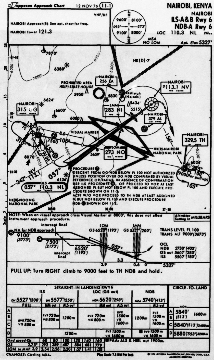
FIGURE 3. RUNWAY APPROACH PLATE
