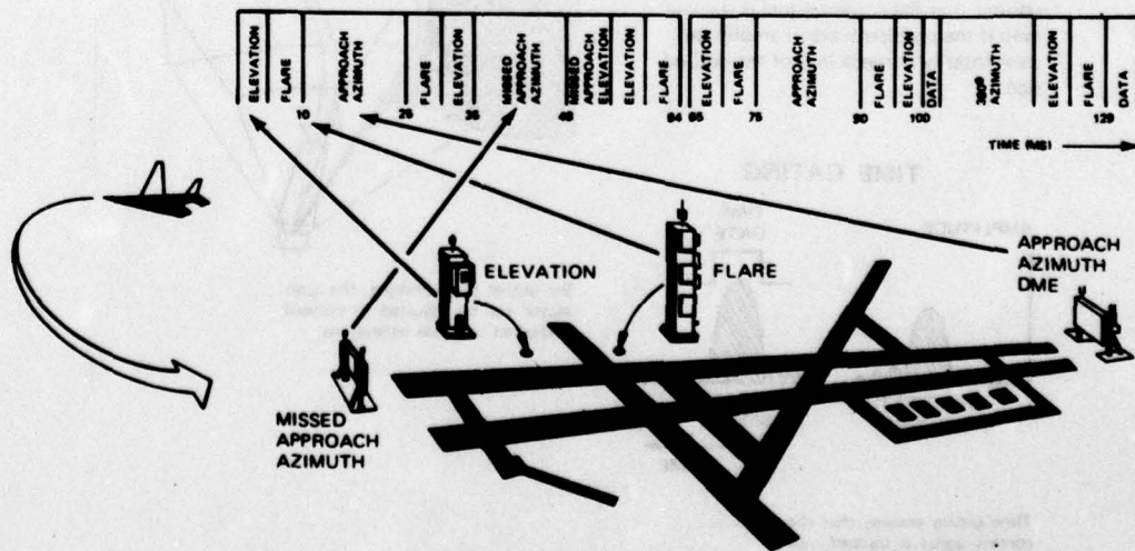
The TRSB signal offers maximum flexibility to meet unique user requirements
