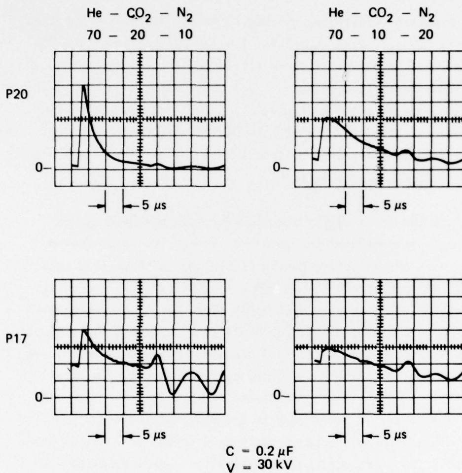
FIGURE 2 - Temporal behavior of the small-signal gain of the regular P20 and of the sequence P17 for two different gas mixtures.
