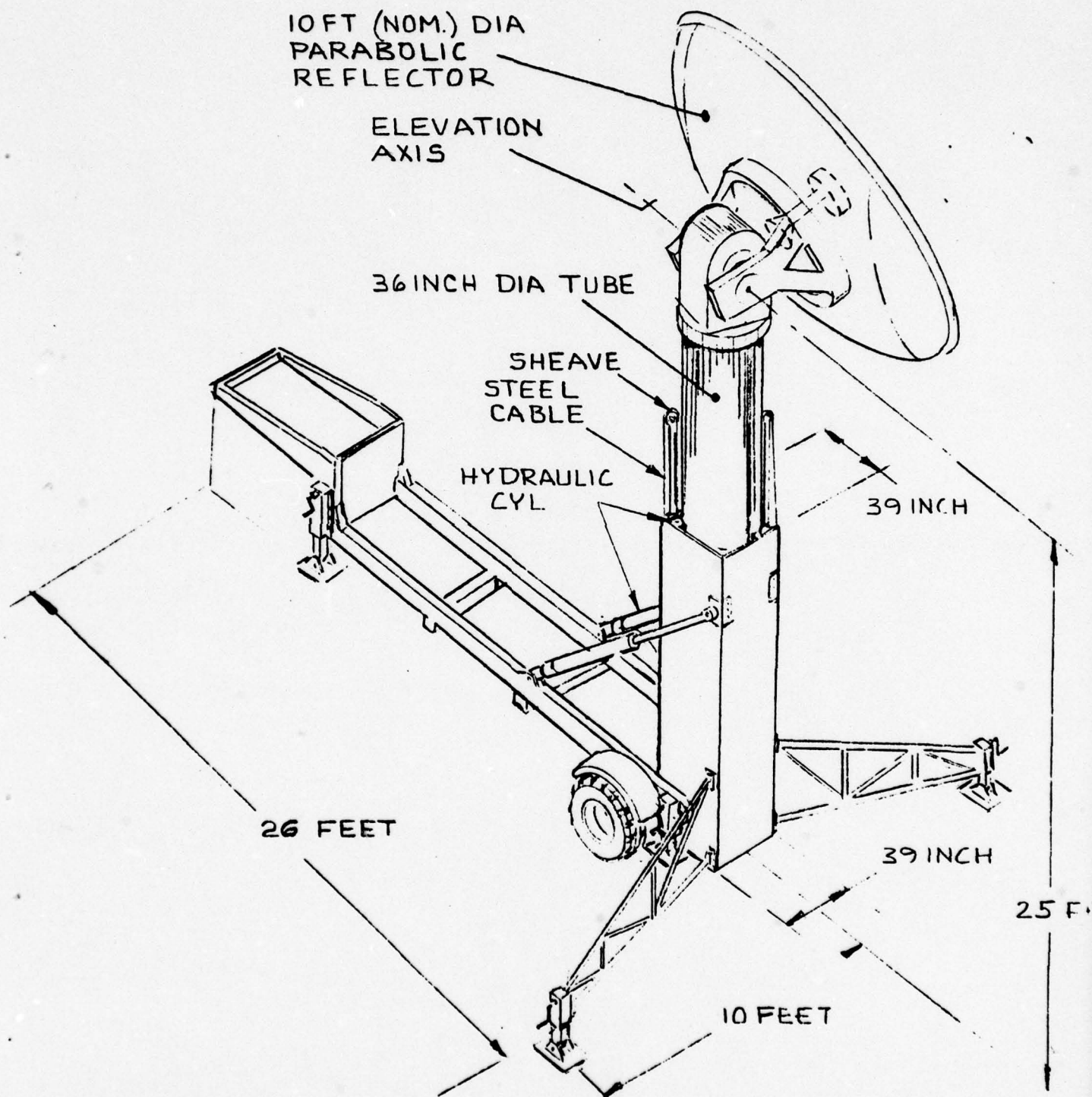
Figure 5.9 FLAT BED TRAILER, MOUNTED ANTENNA, OPERATION MODE
