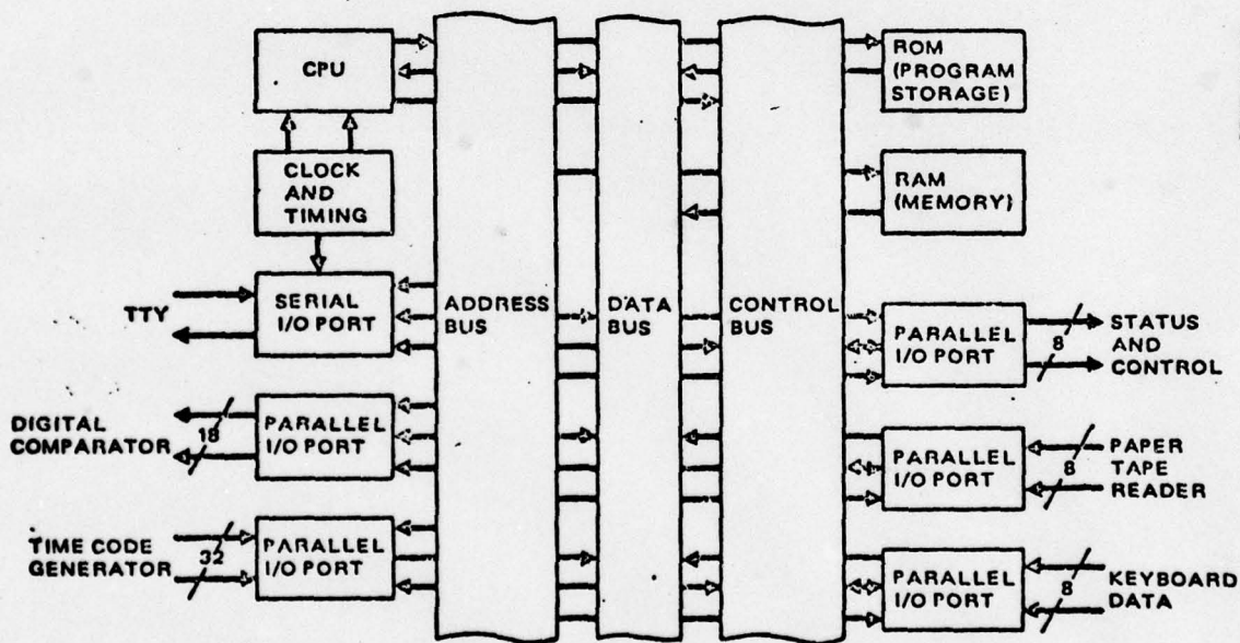
Figure 6.4 ANTENNA PROGRAMMER BLOCK DIAGRAM
