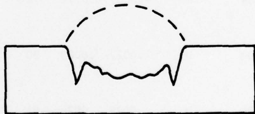
Figure 1. Types of attack between metals and ceramic.
