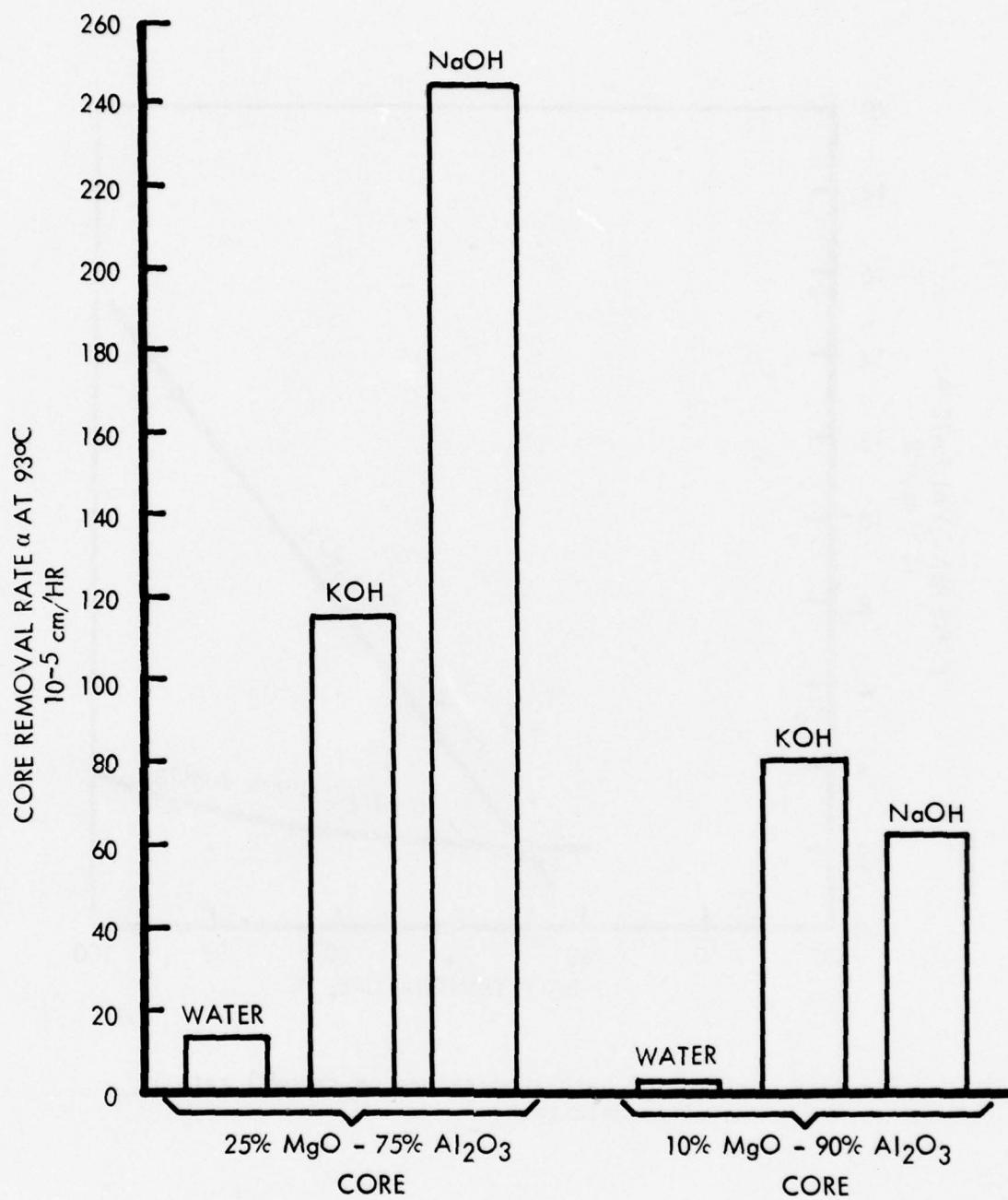
Figure 5. Effect of caustic solutions on removal rate in an ultrasonic bath.
