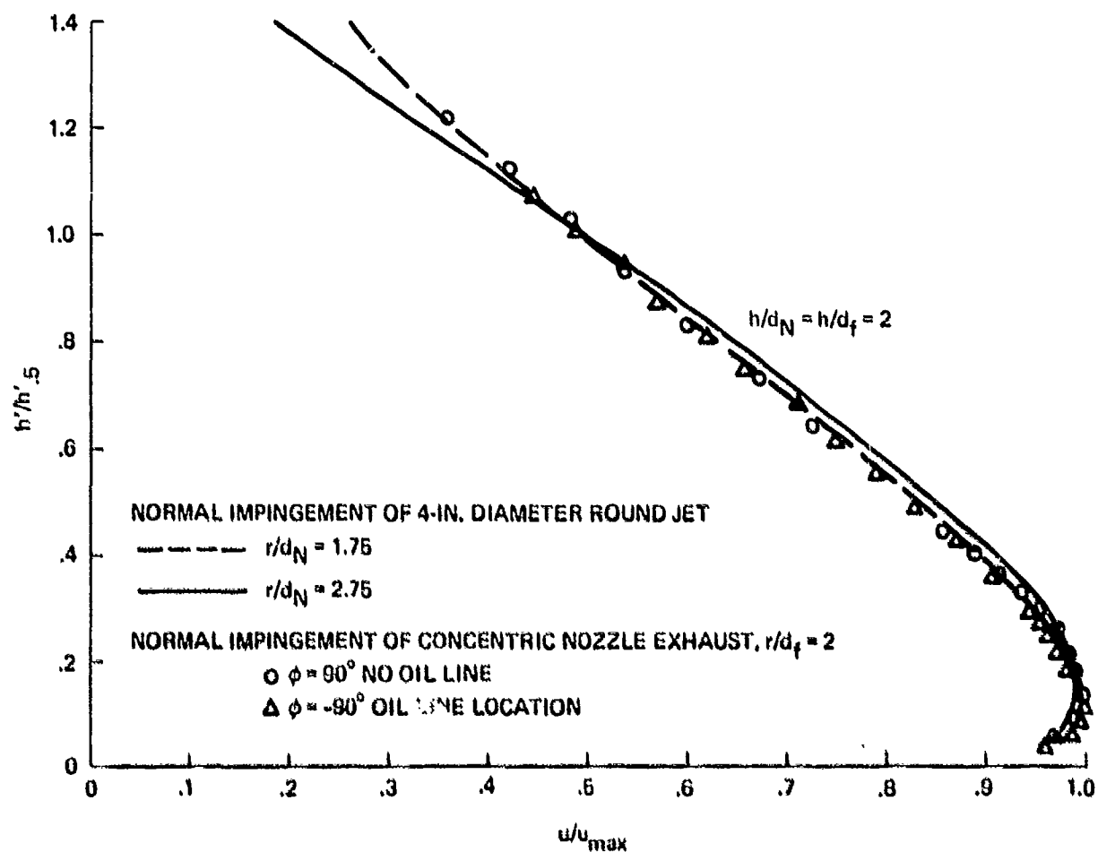
Figure 6 Comparison of Wall Jet Velocity Profiles
