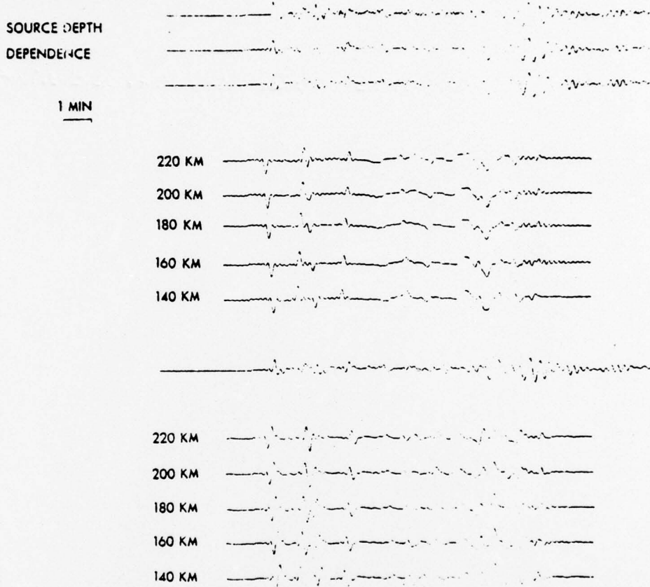
FIG. 2. Dependence of computed seismograms on source depth, which is given at the left of each theoretical seismogram. See caption of Figure 1 for further details.
