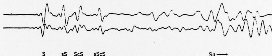
FIG. 5. Best fit to experimental seismogram (lower trace) from theoretical traces shown in Figures 1 to 3, i.e., that with \delta = 90^\circ , \phi = 40^\circ , h = 140 km, \psi = 90^\circ . East is downward.
