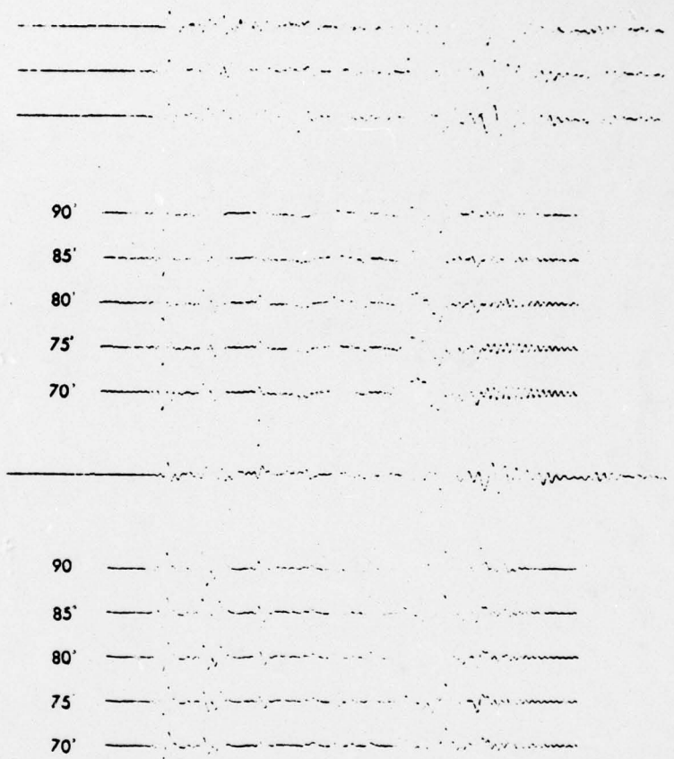
FIG. 1. Dependence of computed seismograms on dip angle at the source. For contrast, the experimental traces extend further to the left and right, and the dominant eastward lobe of the first arrival—S—is upward; on the shorter, theoretical seismograms, eastward is down. Each trace is normalized relative to its maximum displacement from zero. From the top down, the experimental traces show the E-W long-period seismogram at HNR with the ramp function removed, then with a low-pass frequency filter applied (cutoff at 0.1 Hz) after ramp removal, and the lower two also have a Gaussian roll-off filter applied. In Figures 1 to 3 we show the effects of varying source parameters from an initial focal mechanism: dip angle of the fault plane below the horizontal, \delta , of 90^\circ ; azimuthal angle between strike line and epicenter-to-station line, \phi , of 40^\circ ; source depth, h , is initially set at 180 km (Kausel et al. 1977, give the reason for this initial choice of source depth); slip angle of the hanging wall relative to the foot wall, \lambda , of 90^\circ ; and, a step-function displacement dislocation is assumed at the focus, where a point source is assumed, as well as a component of stress, normal to the fault plane, which is continuous during the dislocation. [See Figure 2, Kausel et al. (1977) for fault plane geometry.] In the above figure, the associated dip angle is given at the left of each theoretical trace; the upper group of these time series represents actual ground displacement, and the lower set includes instrumental response [the 30 to 100 instrument described by Knopoff et al. (1973)] and Gaussian roll-off filter.
