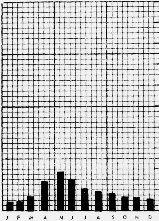
TRAPPING
