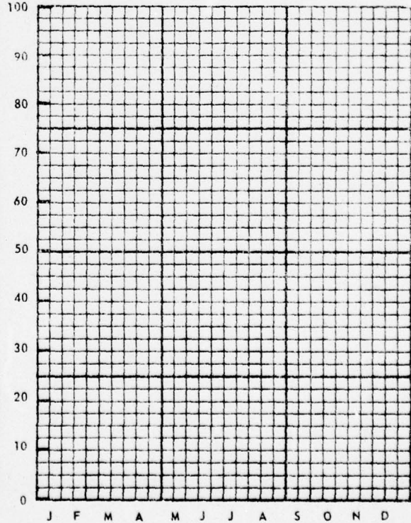
SUBREFRACTIVE
