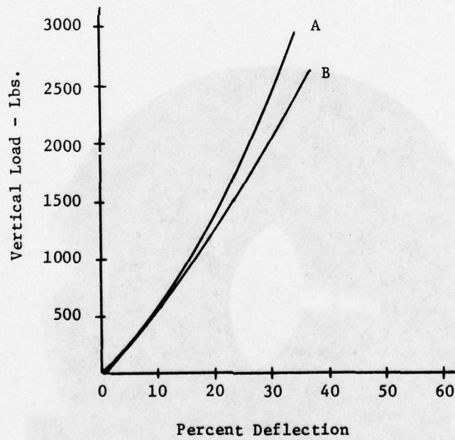
Figure 32 Static Measurements of Cast Tires of Design 74E003A
