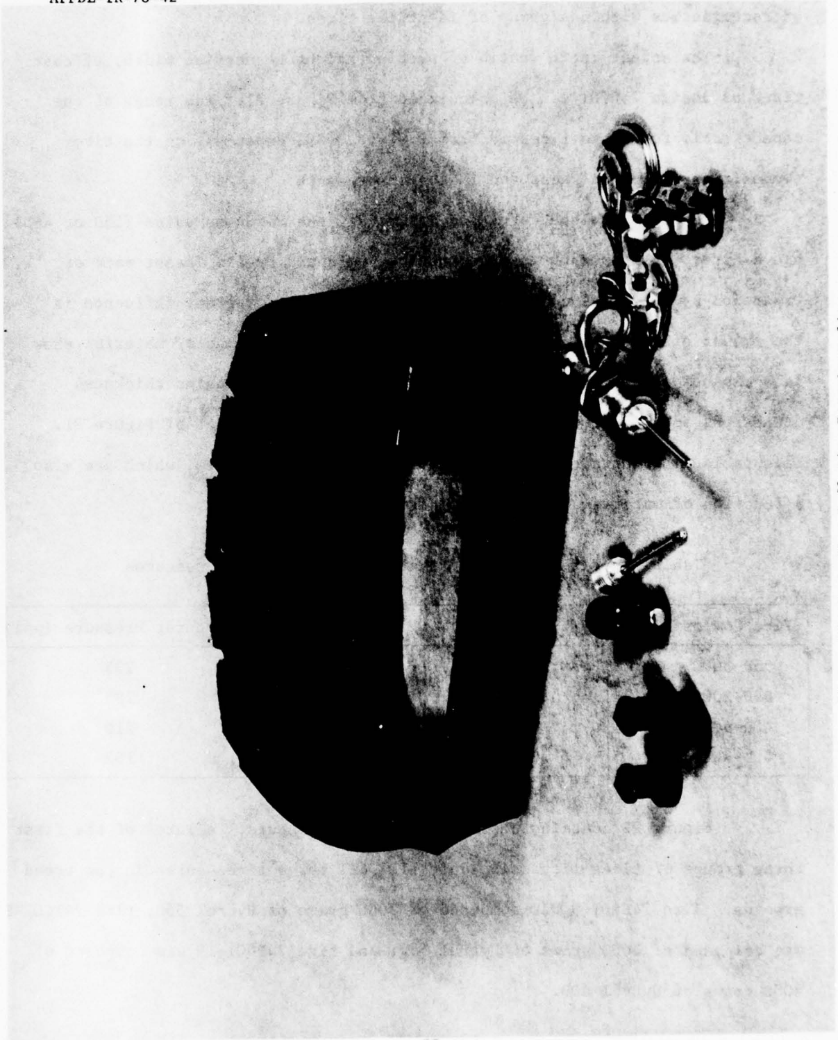
Figure 20 Cast Tire Inflation Paraphernalia
