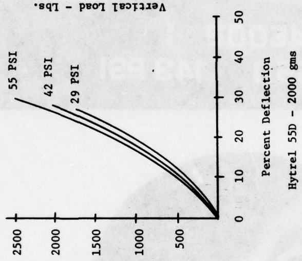
Figure 28 Load vs. Deflection of Cast Tires of Design 74E002
