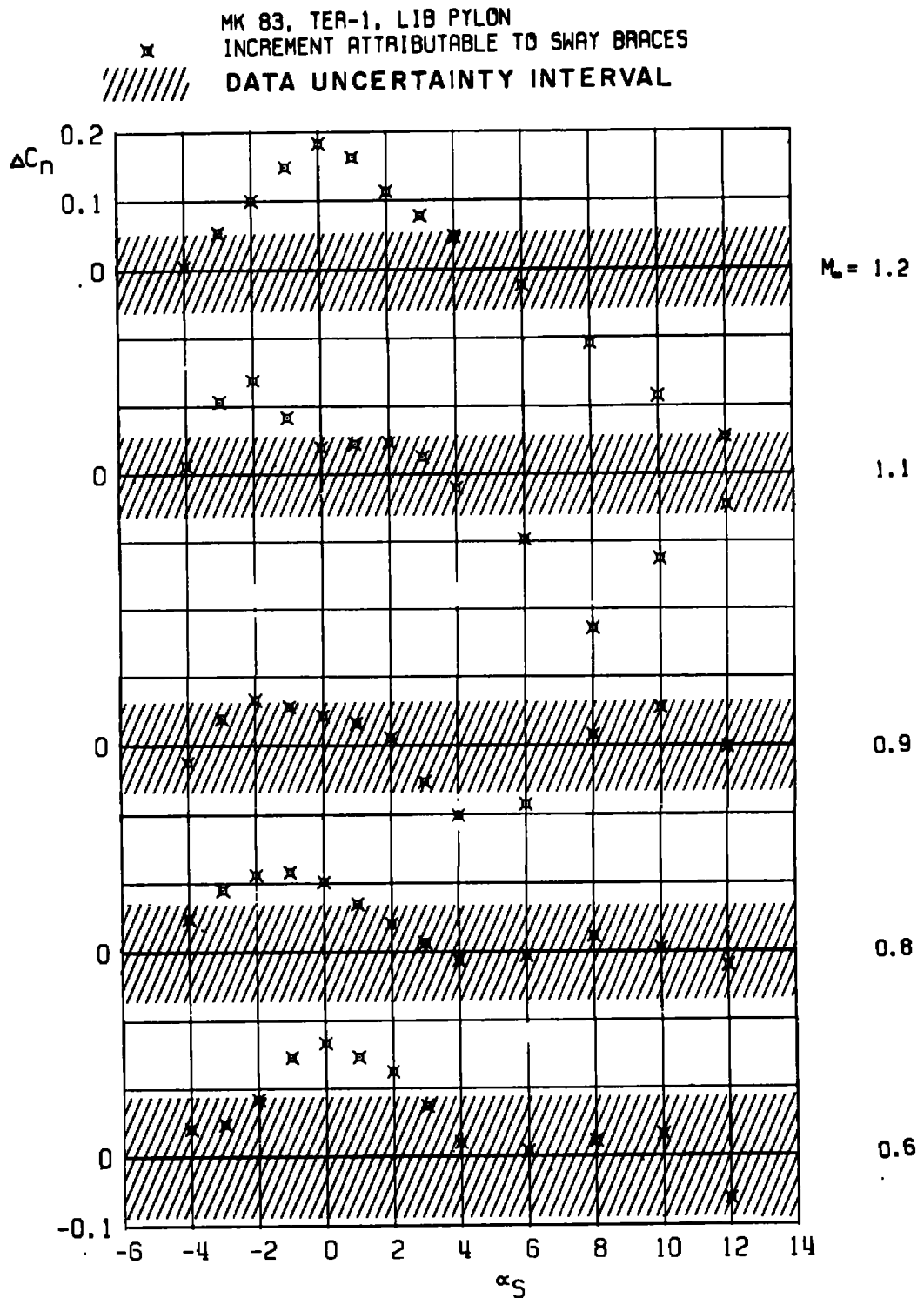
I. Increment in yawing-moment coefficient Figure 18. Concluded.
