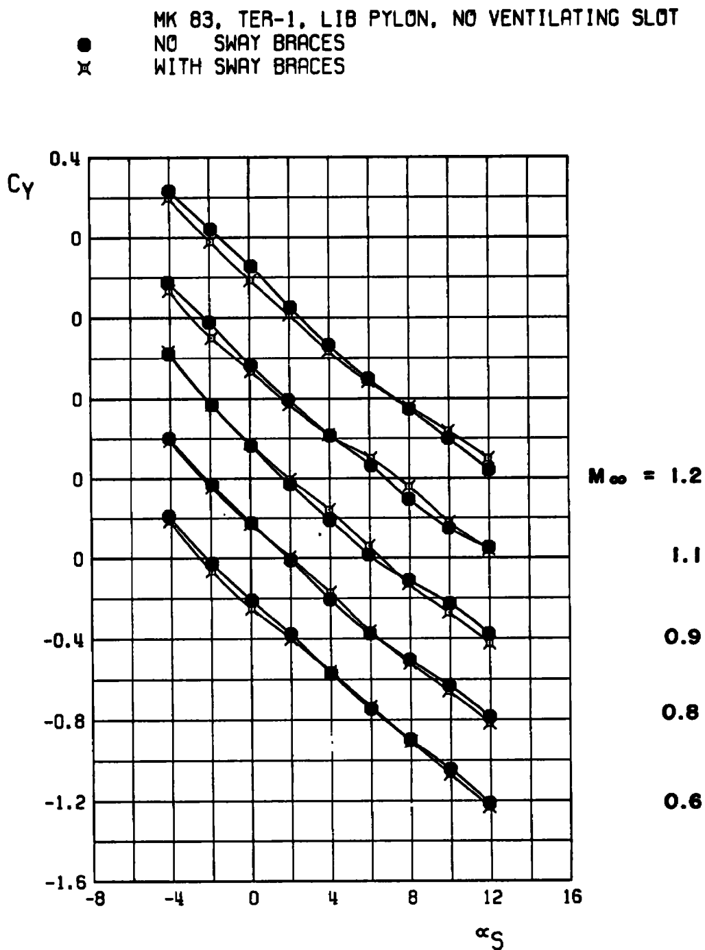
c. Side-force coefficient Figure 18. Continued.
