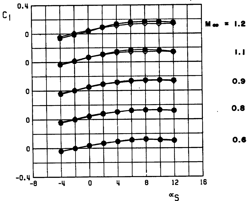
g. Rolling-moment coefficient Figure 16. Continued.
