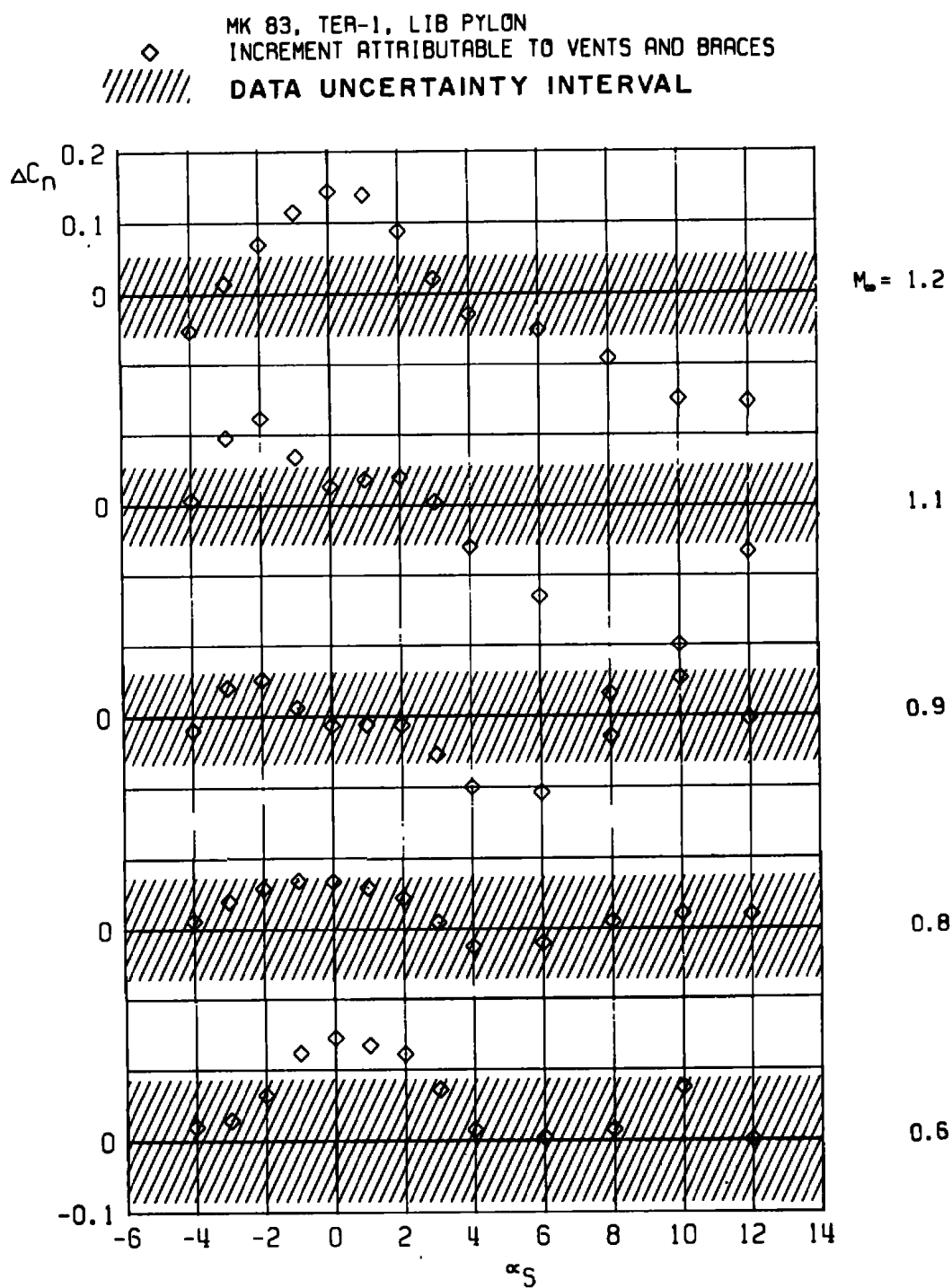
I. Increment in yawing-moment coefficient Figure 19. Concluded.
