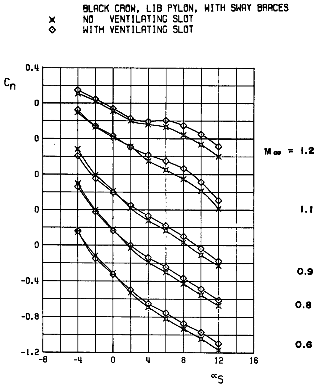
k. Yawing-moment coefficient Figure 12. Continued.
