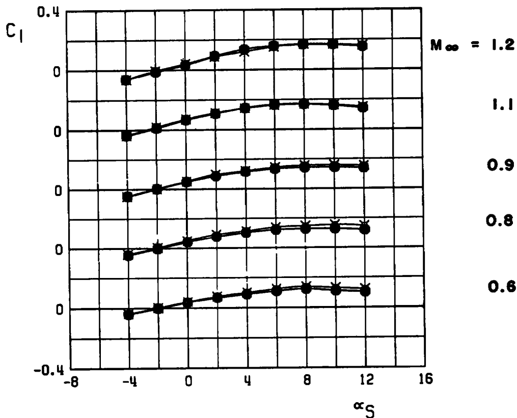
g. Rolling-moment coefficient Figure 15. Continued.
