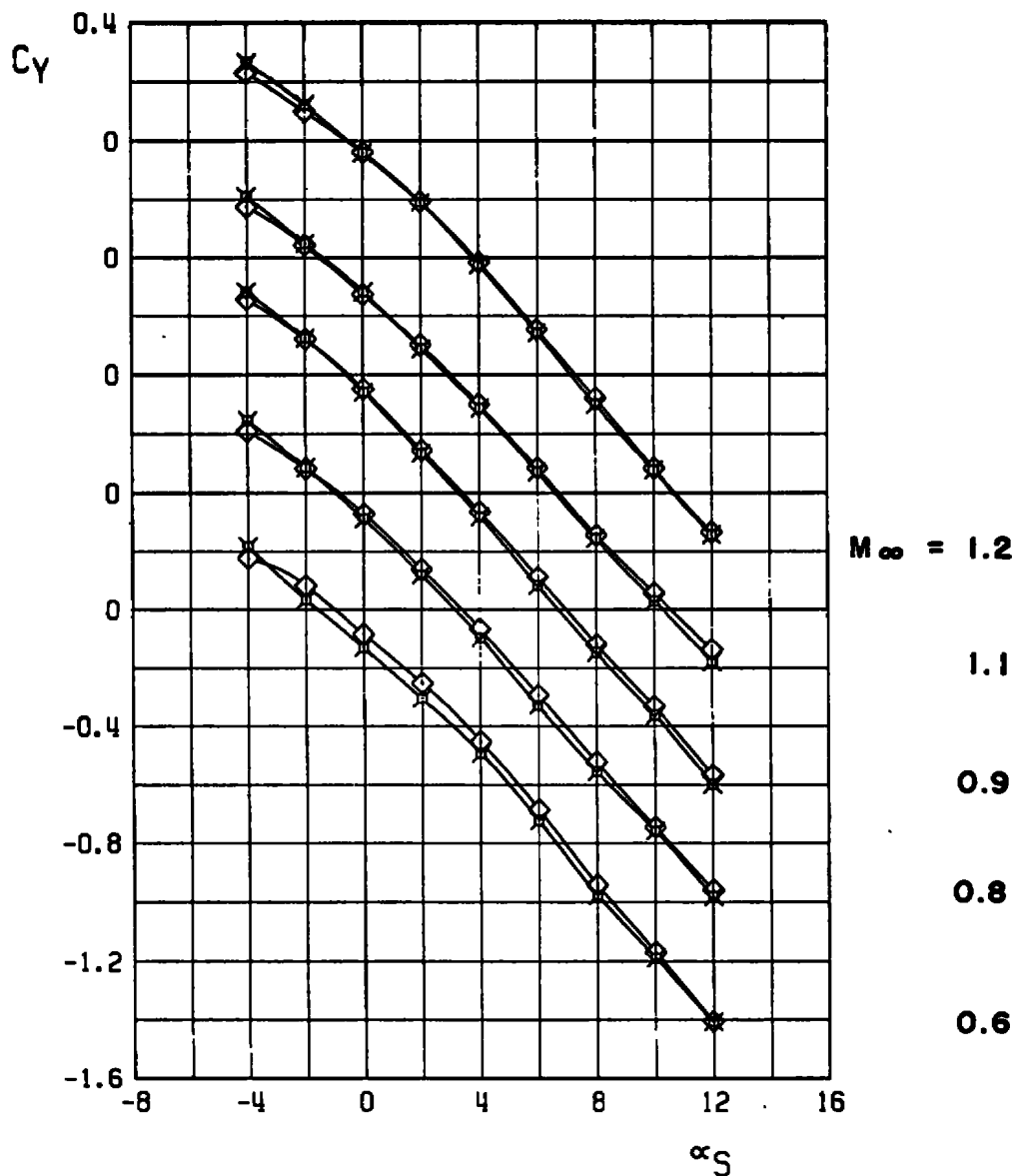
c. Side-force coefficient Figure 12. Continued.
