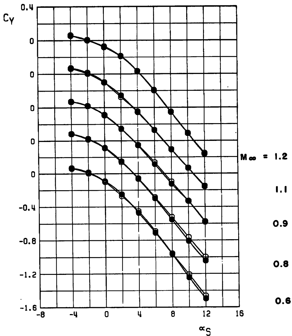
c. Side-force coefficient Figure 14. Continued.
