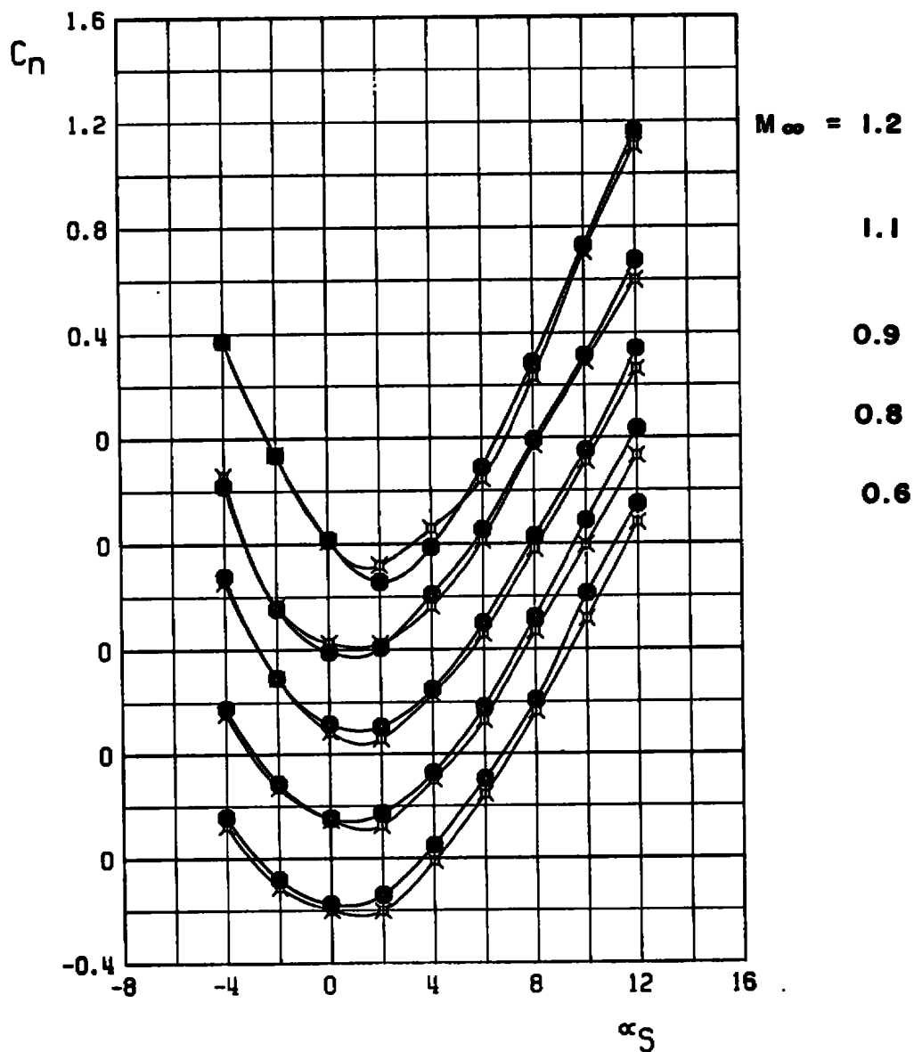
k. Yawing-moment coefficient Figure 15. Continued.
