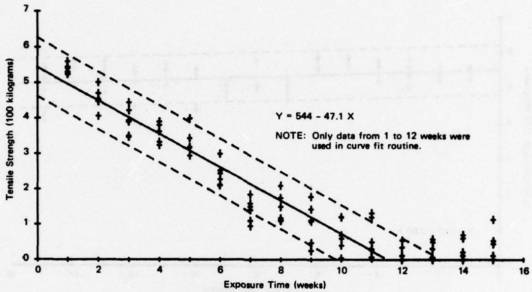
Figure A-7. Steel Strength—Galeta Point Mangrove—Wet Season.
