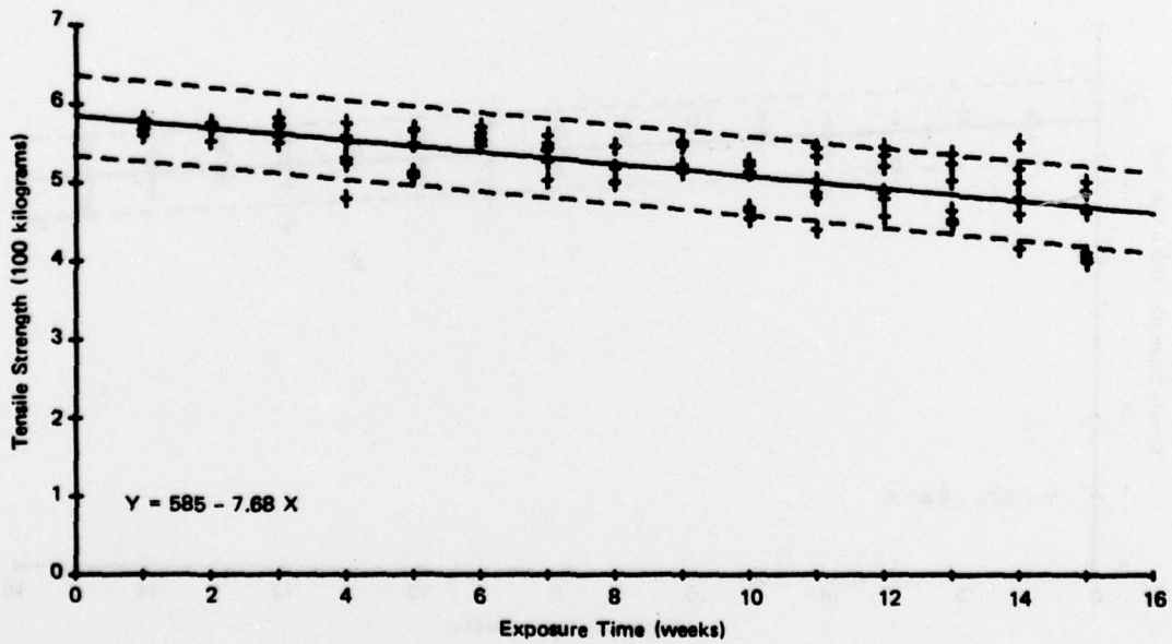
Figure A-14. Steel Strength—Sherman Mangrove B—Dry Season.
