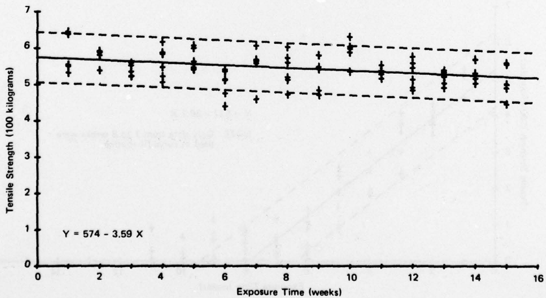
Figure A-10. Steel Strength—Galeta Point Mangrove—Dry Season.
