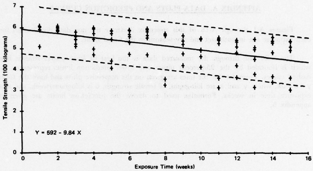
Figure A-1. Steel Strength—Kobbe Mangrove—Wet Season.
