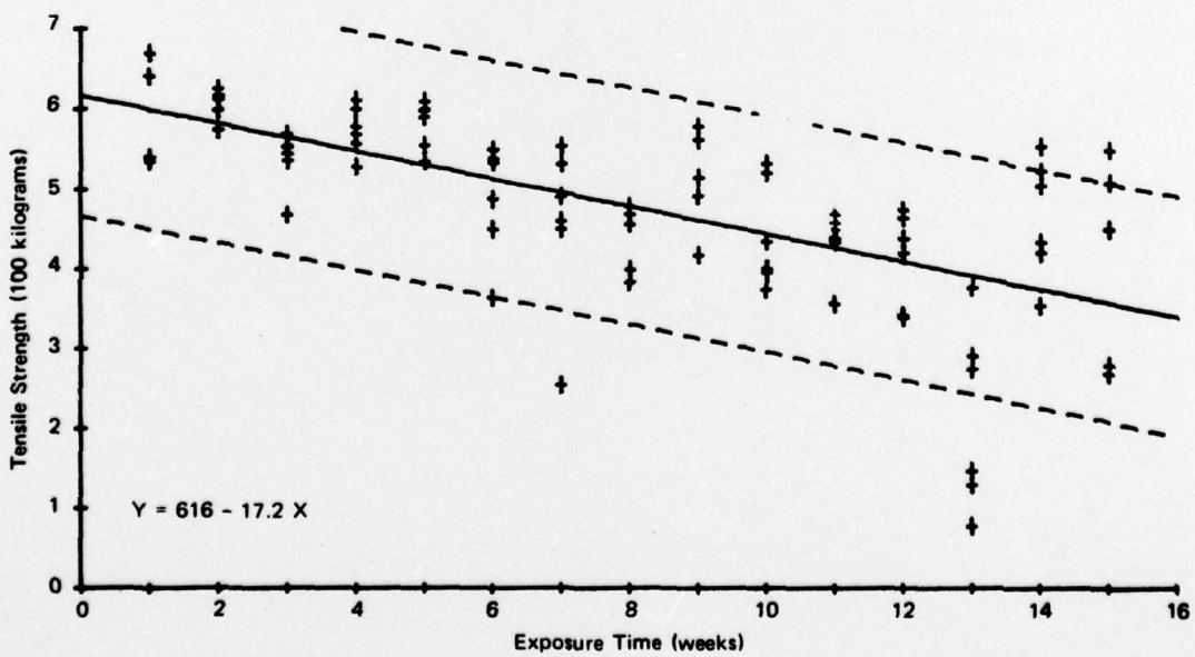
Figure A-2. Steel Strength—Sherman Mangrove A—Wet Season.
