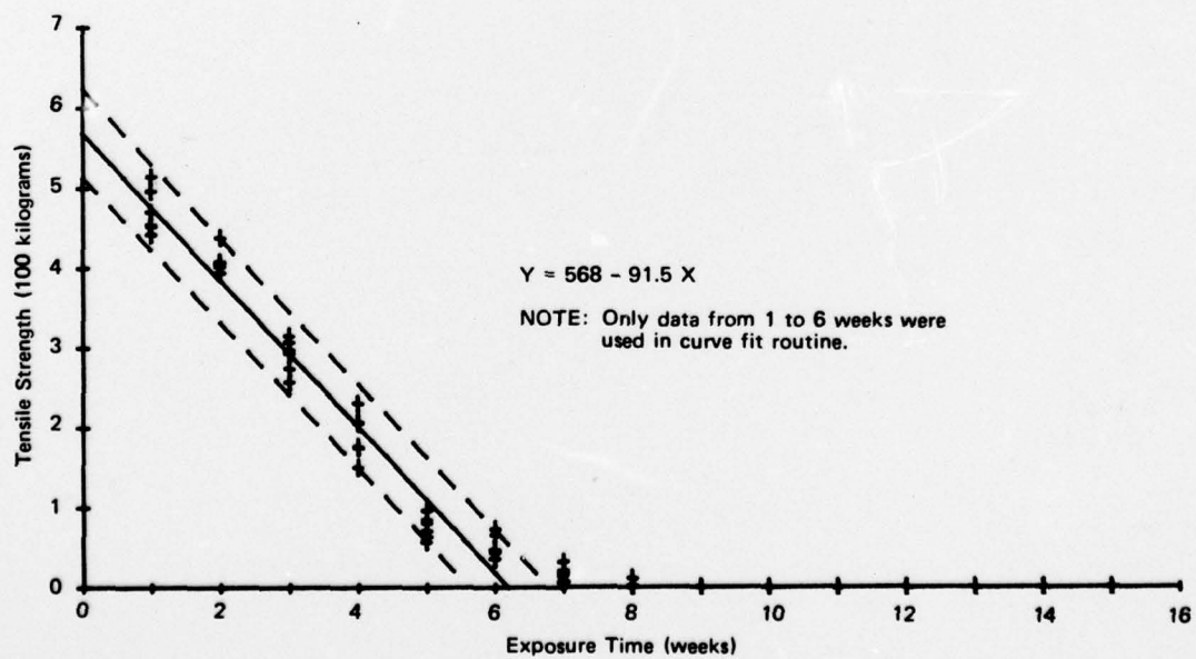
Figure A-16. Steel Strength—Breakwater—Dry Season.
