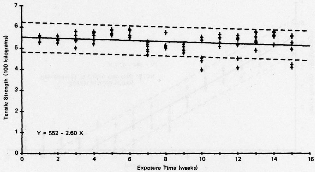
Figure A-9. Steel Strength—Kobbe Mangrove—Dry Season.
