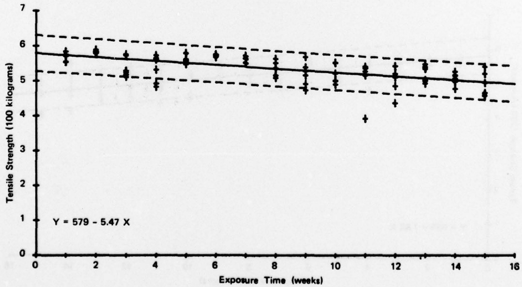
Figure A-12. Steel Strength—Sherman Mangrove A—Dry Season.
