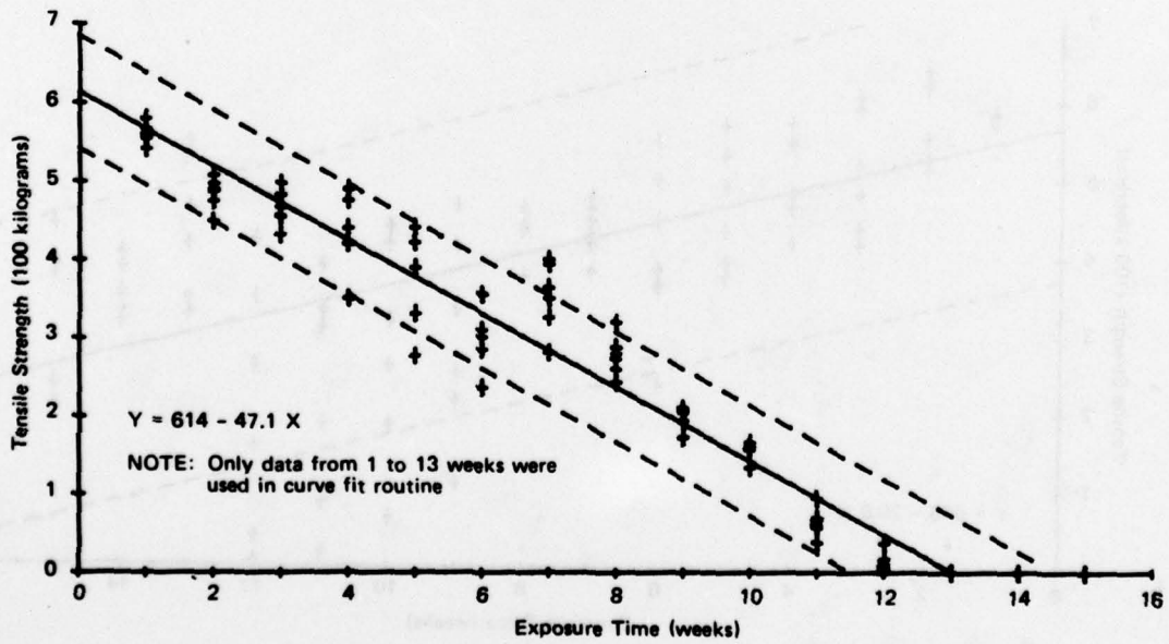
Figure A-6. Steel Strength-Breakwater-Wet Season.
