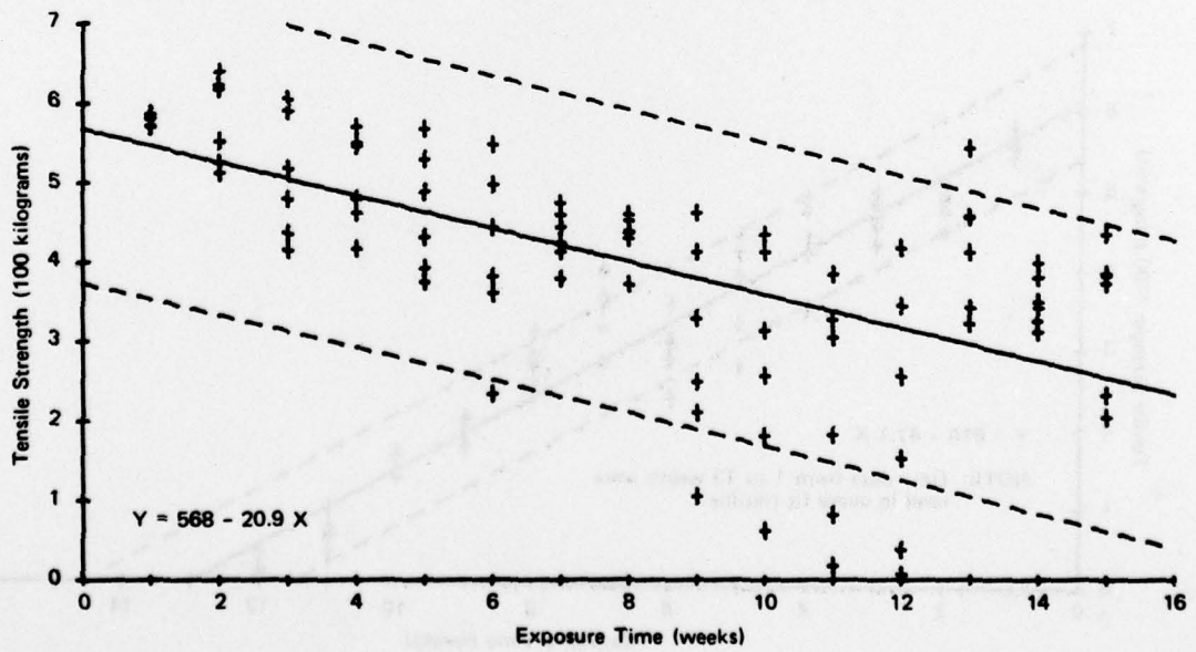
Figure A-4. Steel Strength—Sherman Mangrove B—Wet Season.
