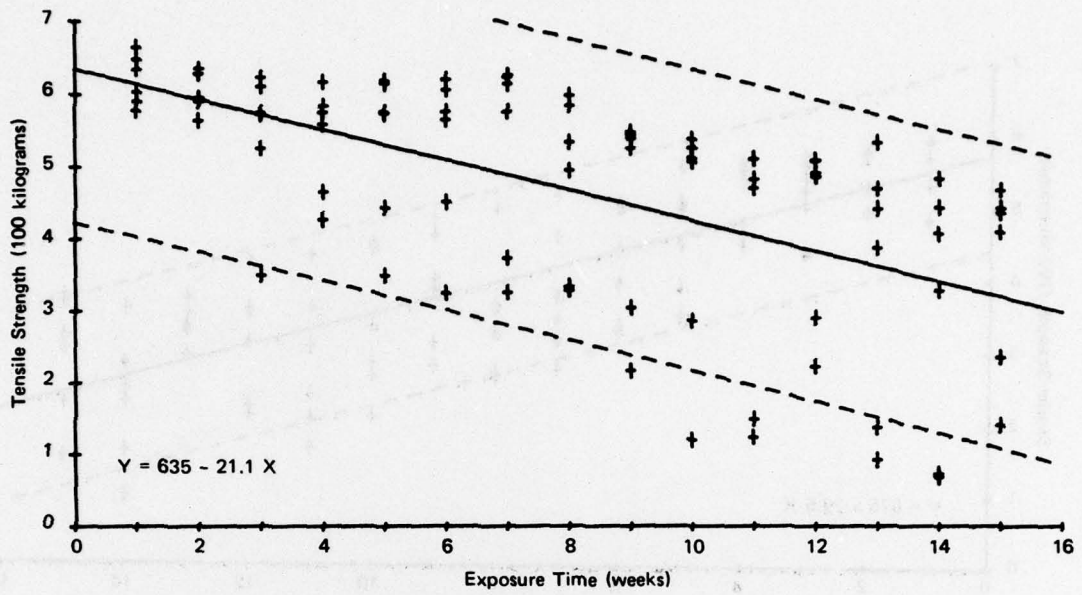
Figure A-3. Steel Strength—Rodman Mangrove—Wet Season.
