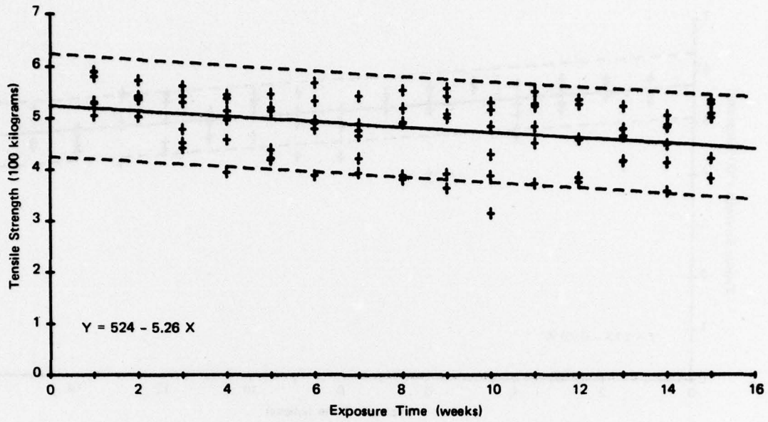
Figure A-11. Steel Strength—Rodman Mangrove—Dry Season.
