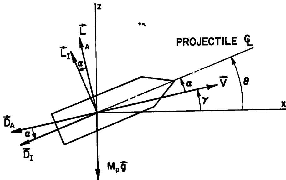
Figure 16. Forces Acting on the Projectile.
