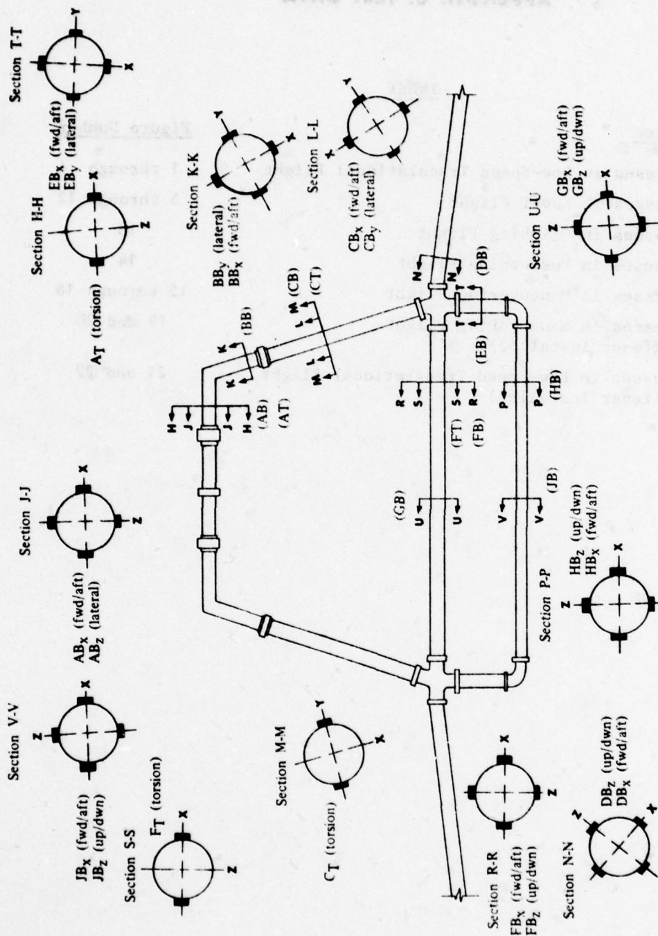
Figure 1. Spray Boom Instrumentation Schematic
