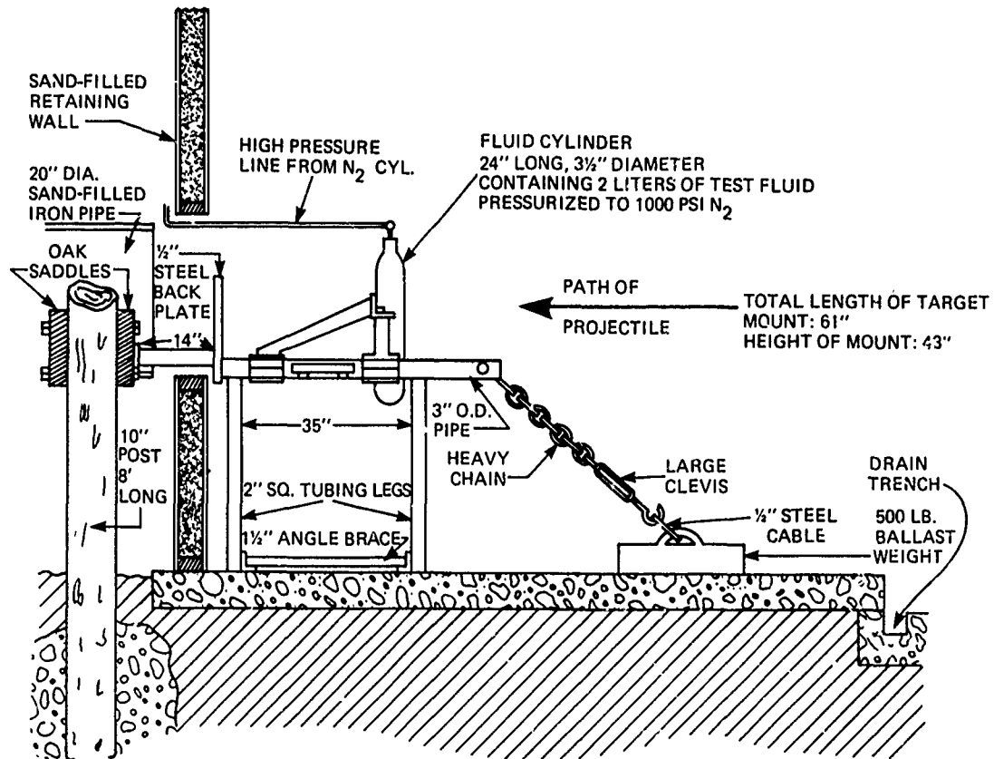
FIGURE 3. ILLUSTRATION OF HYDRAULIC CYLINDER TARGET ASSEMBLY
