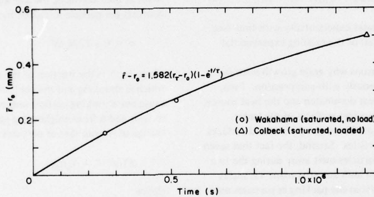
Figure 3. The increase in grain radius shown with time for r_r = 1 mm and \tau = 1,209,600 s.
