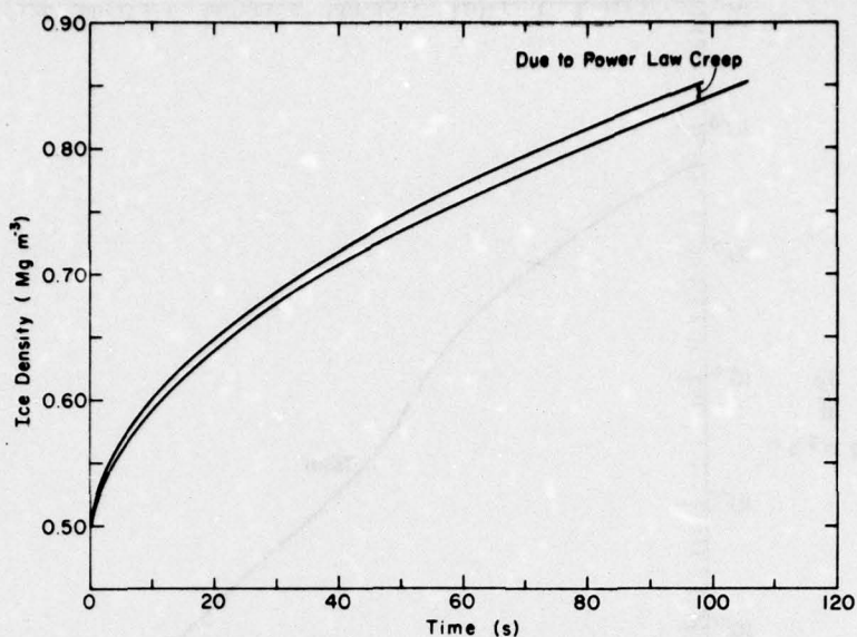
Figure 10. The ice density shown against time for reglation plus nonlinear viscous creep and reglation alone. The difference between the two lines is the contribution of the power law creep.
