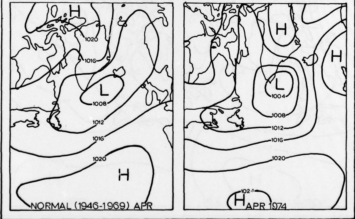
Figure 26d.—April Normal and 1974 Monthly Average Surface Pressure in mbs Relative to 1000 mbs.
