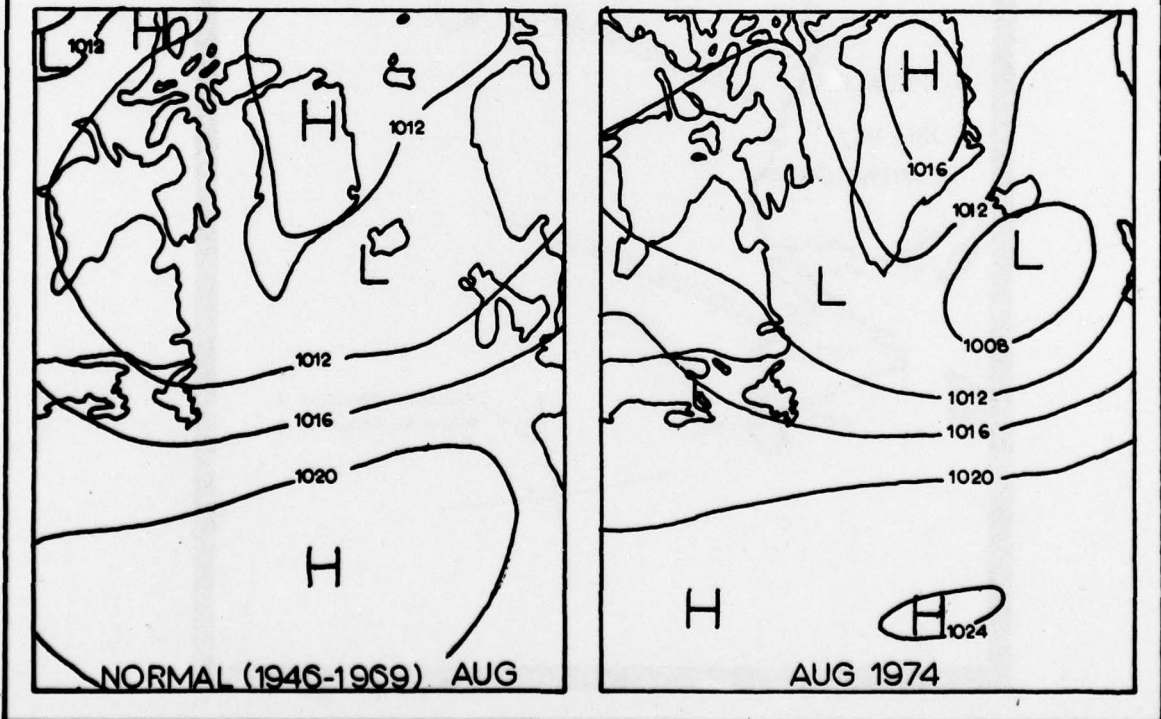
Figure 26h.—August Normal and 1974 Monthly Average Surface Pressure in mbs Relative to 1000 mbs.
