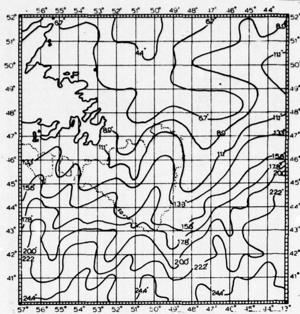
FIGURE C-1.—Mean Sea Surface Temperature for July.
