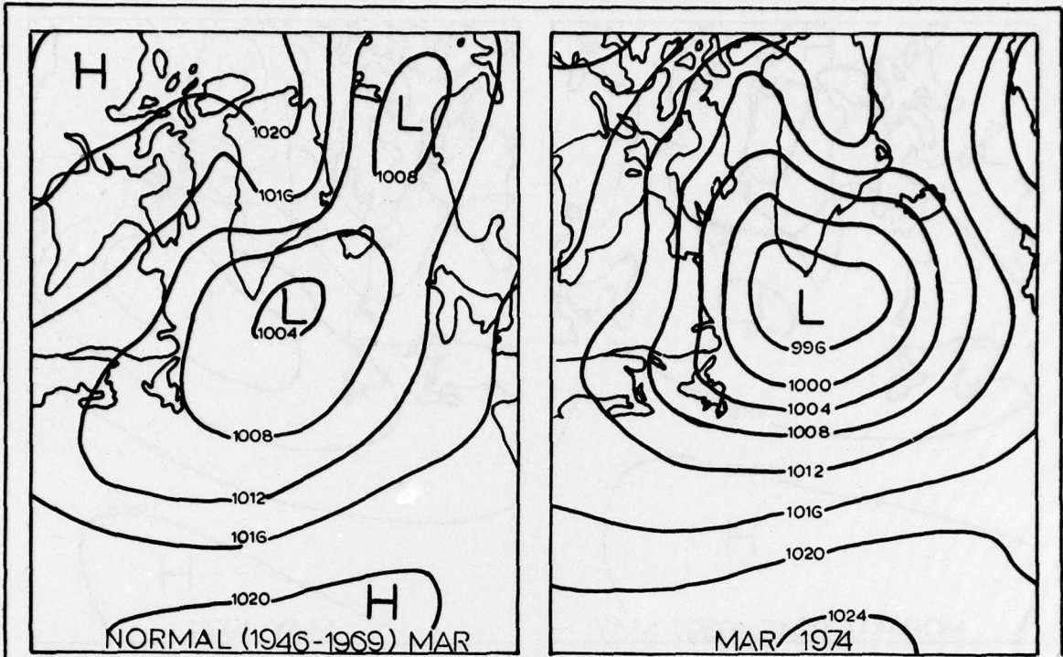
Figure 26c.—March Normal and 1974 Monthly Average Surface Pressure in mbs Relative to 1000 mbs.
