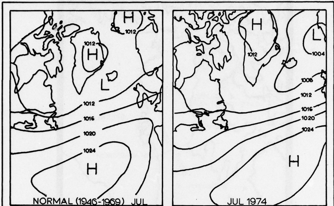
Figure 26g.—July Normal and 1974 Monthly Average Surface Pressure in mbs Relative to 1000 mbs.
