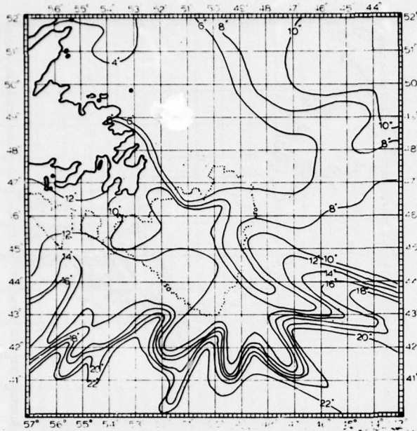
FIGURE C-5.—SST Marcom, Halifax, 18 to 21 July 1974.
