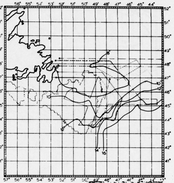
FIGURE C-6.—ART SST Flights, 24 to 30 July 1974.
