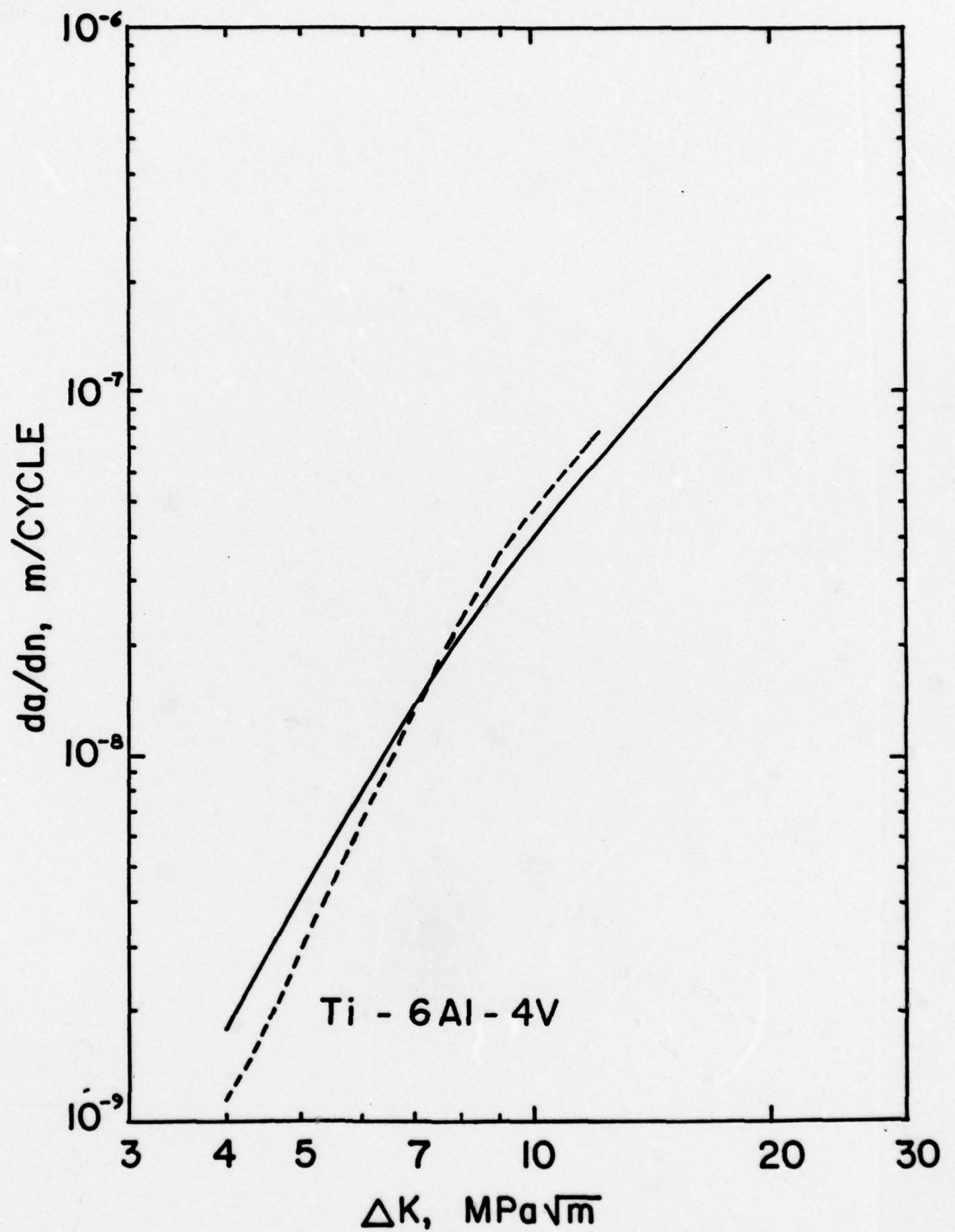
(c) For a Ti-6Al-4V alloy in martensitic condition (29,31) . c = -0.7 , \epsilon_f' = 1 , \sigma_y' = 880 MPa, n' = 0.086 , \rho = 2.5 \mu\text{m} , E = 120 GPa. The calculated FCGR is given by solid lines. The best fit experimental curve (31) is shown by dotted line.
