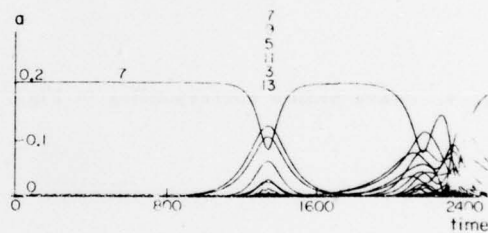
Fig. 10. Instability bursts.
